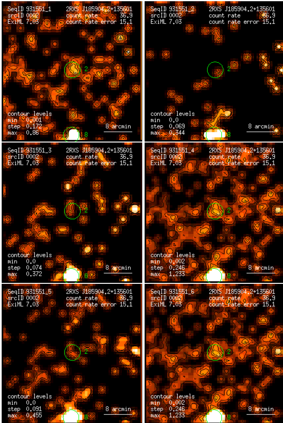
Figure 2: RASS 931551: detection 0002: band rate images, Gaussian filter: (1) PSPC channels 11 – 41, (2) 52 – 90, (3) 91 – 201, (4) 11 – 235, (5) 52 – 201, (6) 11 – 201. Broad band rates in counts/ks. Band rate contour levels in counts/ks/arcmin 2 .
