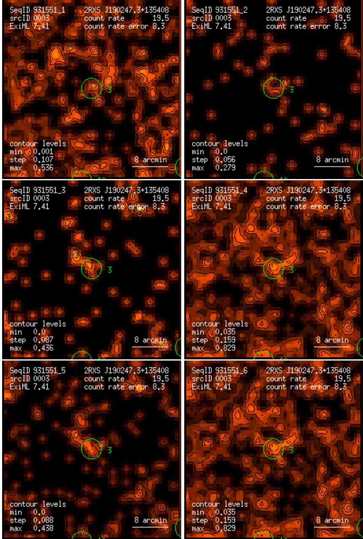
Figure 3: RASS 931551: detection 0003: band rate images, Gaussian filter: (1) PSPC channels 11 – 41, (2) 52 – 90, (3) 91 – 201, (4) 11 – 235, (5) 52 – 201, (6) 11 – 201. Broad band rates in counts/ks. Band rate contour levels in counts/ks/arcmin 2 .
