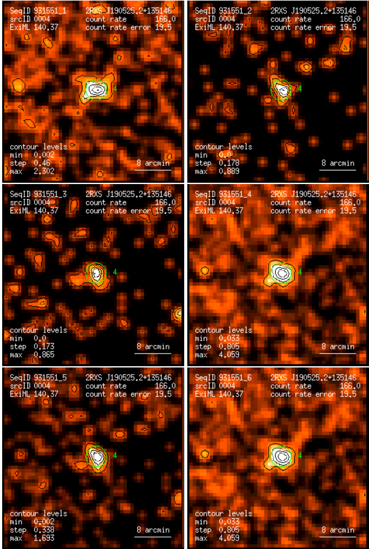
Figure 4: RASS 931551: detection 0004: band rate images, Gaussian filter: (1) PSPC channels 11 – 41, (2) 52 – 90, (3) 91 – 201, (4) 11 – 235, (5) 52 – 201, (6) 11 – 201. Broad band rates in counts/ks. Band rate contour levels in counts/ks/arcmin 2 .
