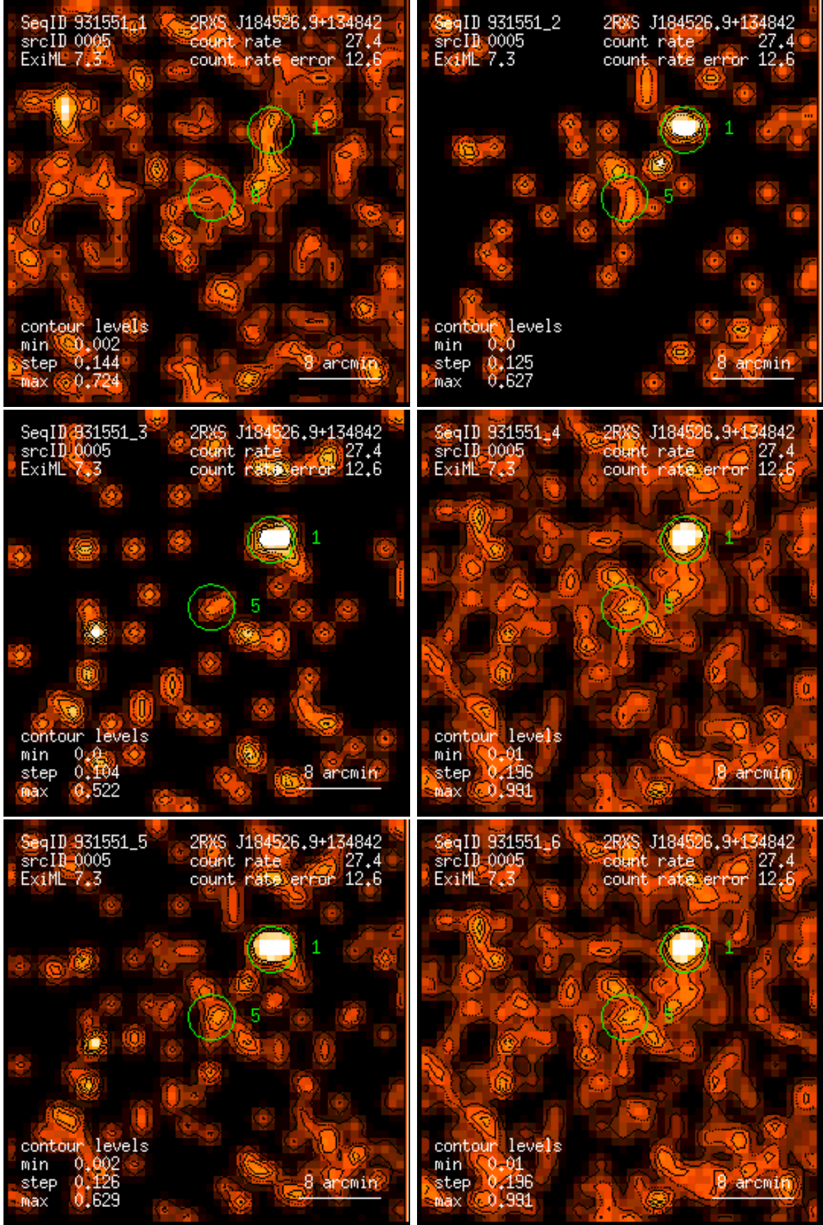
Figure 5: RASS 931551: detection 0005: band rate images, Gaussian filter: (1) PSPC channels 11 – 41, (2) 52 – 90, (3) 91 – 201, (4) 11 – 235, (5) 52 – 201, (6) 11 – 201. Broad band rates in counts/ks. Band rate contour levels in counts/ks/arcmin 2 .
