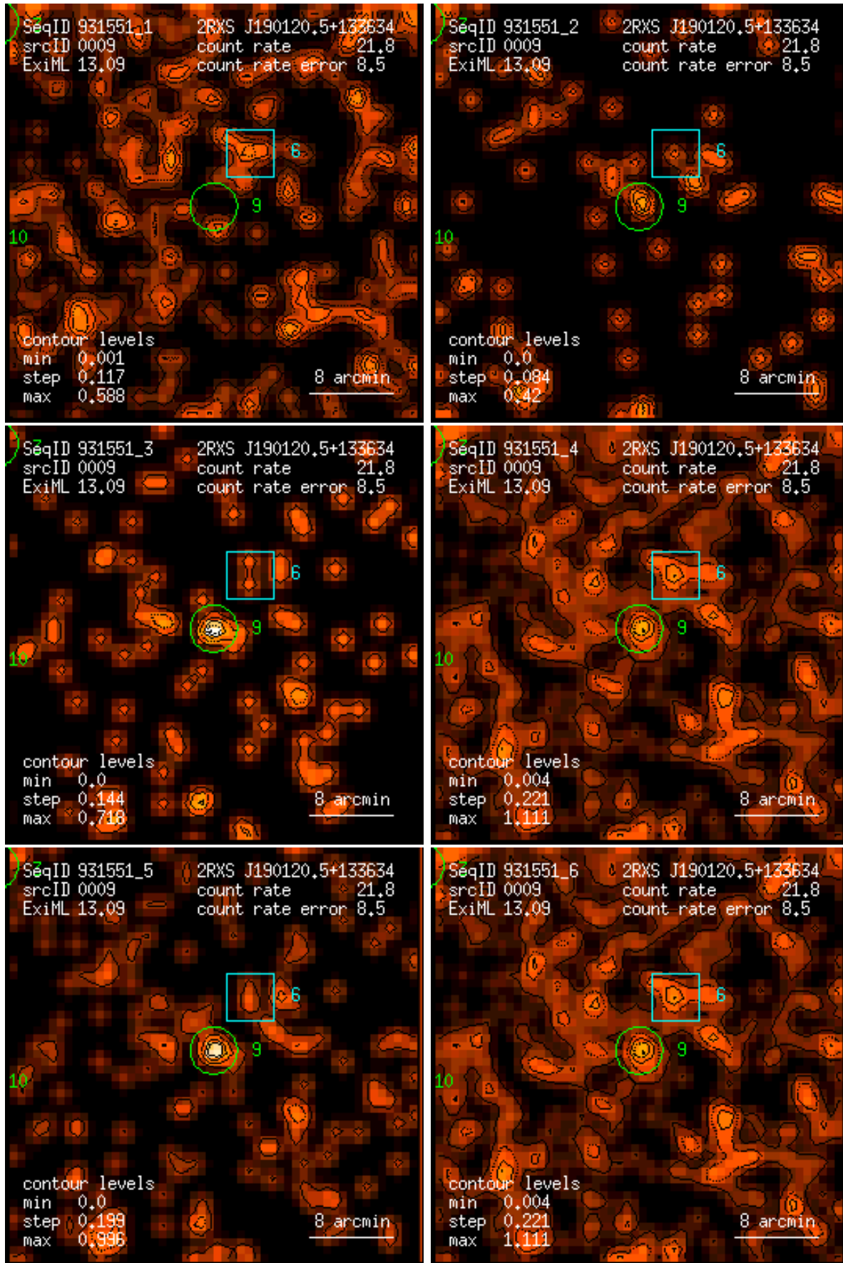
Figure 9: RASS 931551: detection 0009: band rate images, Gaussian filter: (1) PSPC channels 11 – 41, (2) 52 – 90, (3) 91 – 201, (4) 11 – 235, (5) 52 – 201, (6) 11 – 201. Broad band rates in counts/ks. Band rate contour levels in counts/ks/arcmin 2 .
