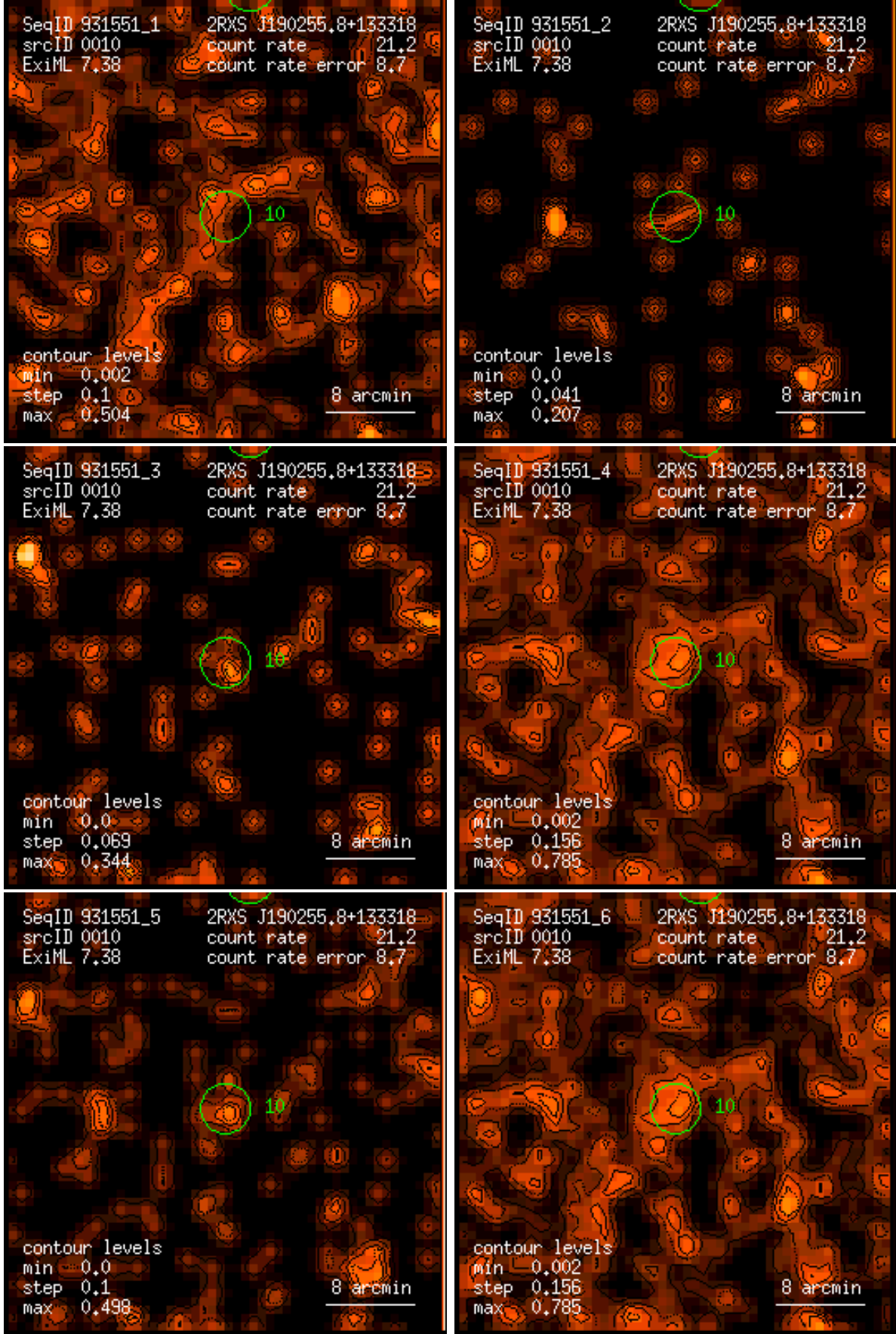
Figure 10: RASS 931551: detection 0010: band rate images, Gaussian filter: (1) PSPC channels 11 – 41, (2) 52 – 90, (3) 91 – 201, (4) 11 – 235, (5) 52 – 201, (6) 11 – 201. Broad band rates in counts/ks. Band rate contour levels in counts/ks/arcmin 2 .
