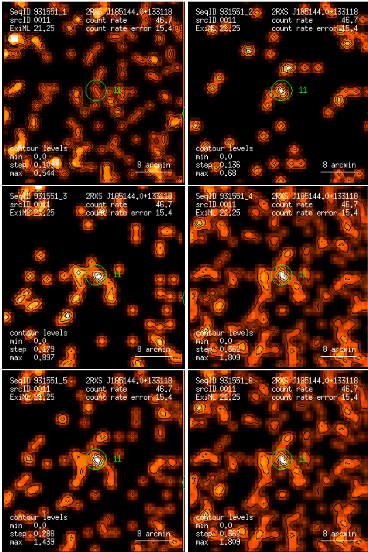
Figure 11: RASS 931551: detection 0011: band rate images, Gaussian filter: (1) PSPC channels 11 – 41, (2) 52 – 90, (3) 91 – 201, (4) 11 – 235, (5) 52 – 201, (6) 11 – 201. Broad band rates in counts/ks. Band rate contour levels in counts/ks/arcmin 2 .
