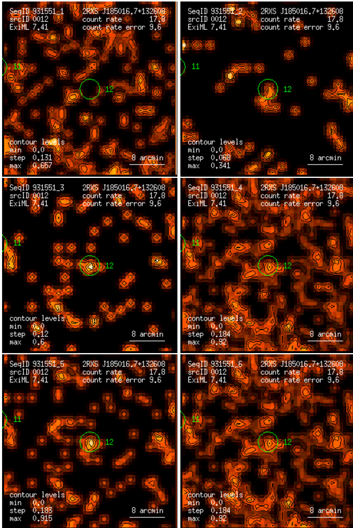
Figure 12: RASS 931551: detection 0012: band rate images, Gaussian filter: (1) PSPC channels 11 – 41, (2) 52 – 90, (3) 91 – 201, (4) 11 – 235, (5) 52 – 201, (6) 11 – 201. Broad band rates in counts/ks. Band rate contour levels in counts/ks/arcmin 2 .
