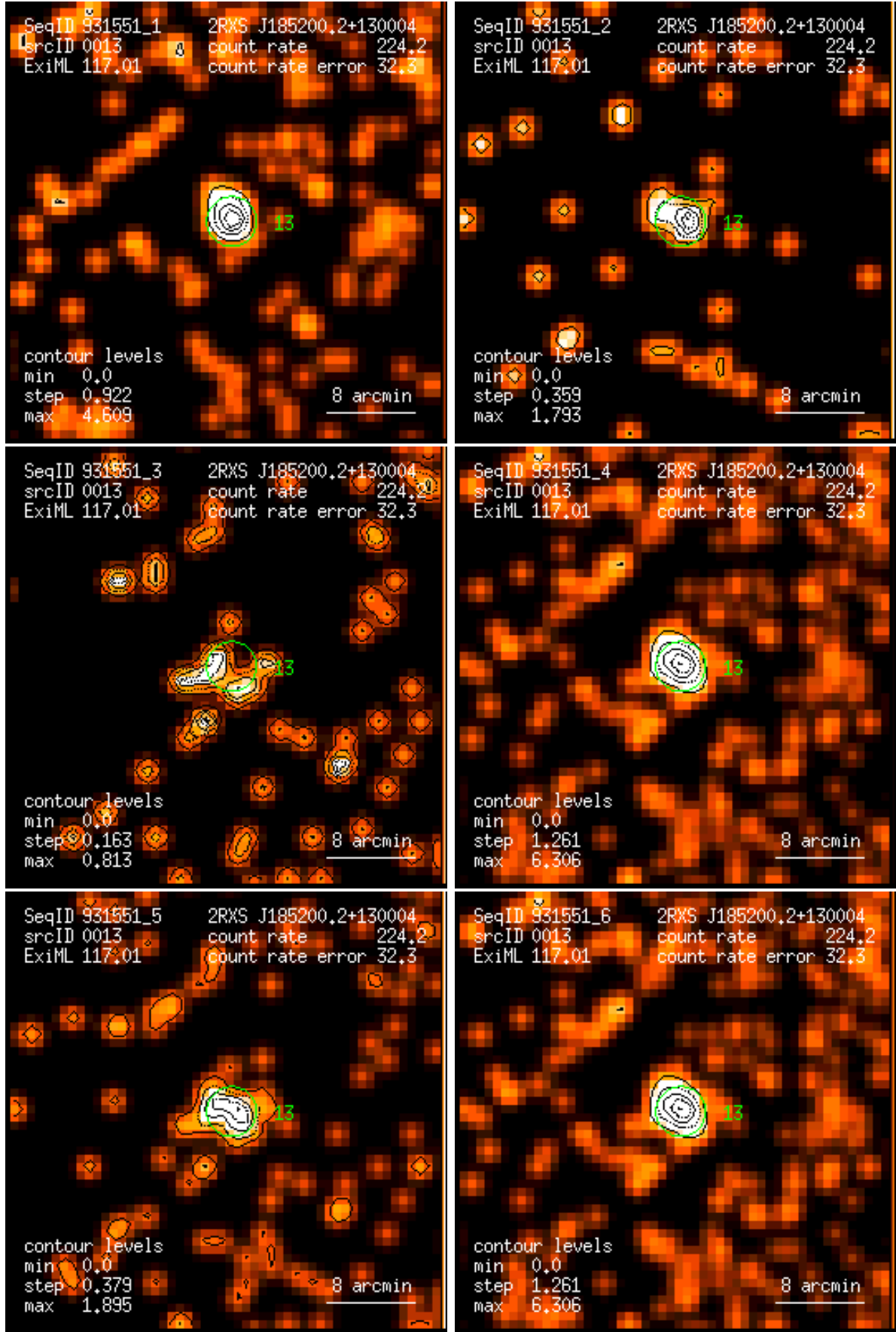
Figure 13: RASS 931551: detection 0013: band rate images, Gaussian filter: (1) PSPC channels 11 – 41, (2) 52 – 90, (3) 91 – 201, (4) 11 – 235, (5) 52 – 201, (6) 11 – 201. Broad band rates in counts/ks. Band rate contour levels in counts/ks/arcmin 2 .
