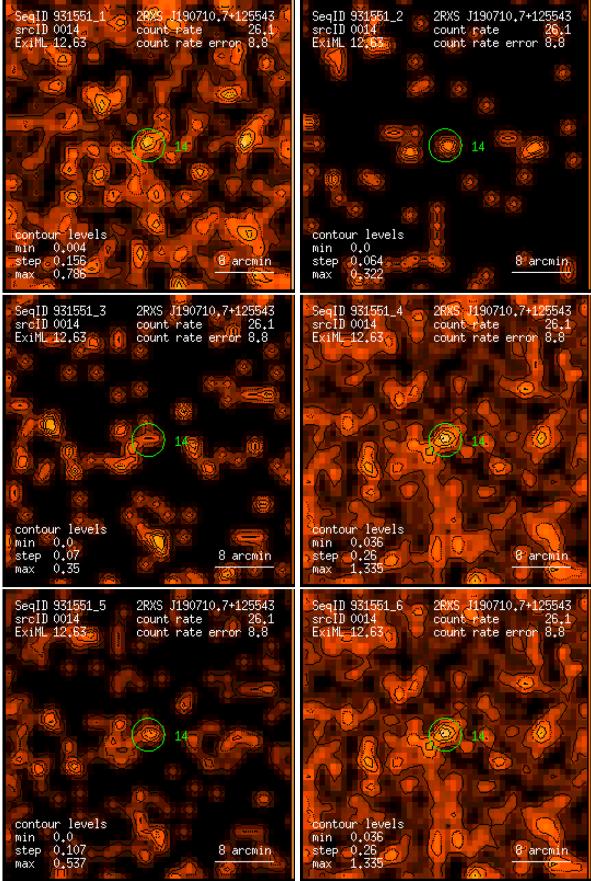
Figure 14: RASS 931551: detection 0014: band rate images, Gaussian filter: (1) PSPC channels 11 – 41, (2) 52 – 90, (3) 91 – 201, (4) 11 – 235, (5) 52 – 201, (6) 11 – 201. Broad band rates in counts/ks. Band rate contour levels in counts/ks/arcmin 2 .
