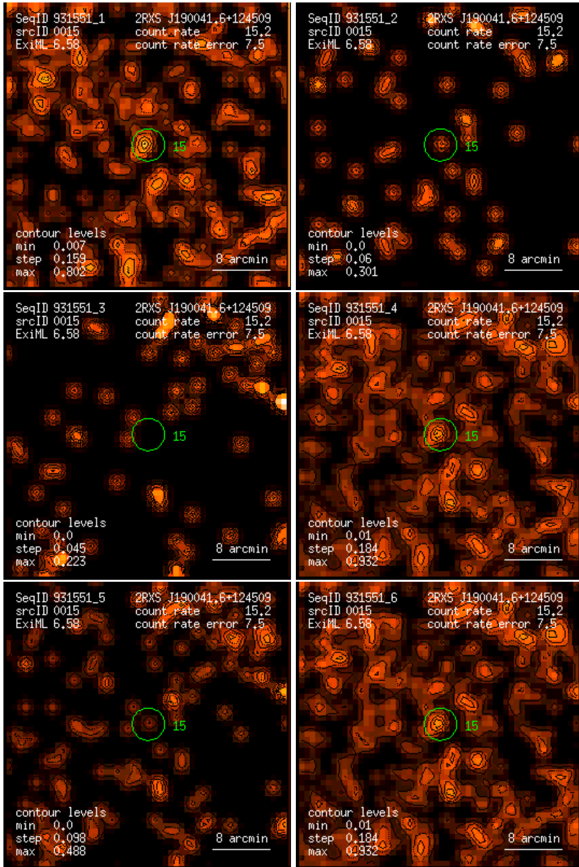
Figure 15: RASS 931551: detection 0015: band rate images, Gaussian filter: (1) PSPC channels 11 – 41, (2) 52 – 90, (3) 91 – 201, (4) 11 – 235, (5) 52 – 201, (6) 11 – 201. Broad band rates in counts/ks. Band rate contour levels in counts/ks/arcmin 2 .
