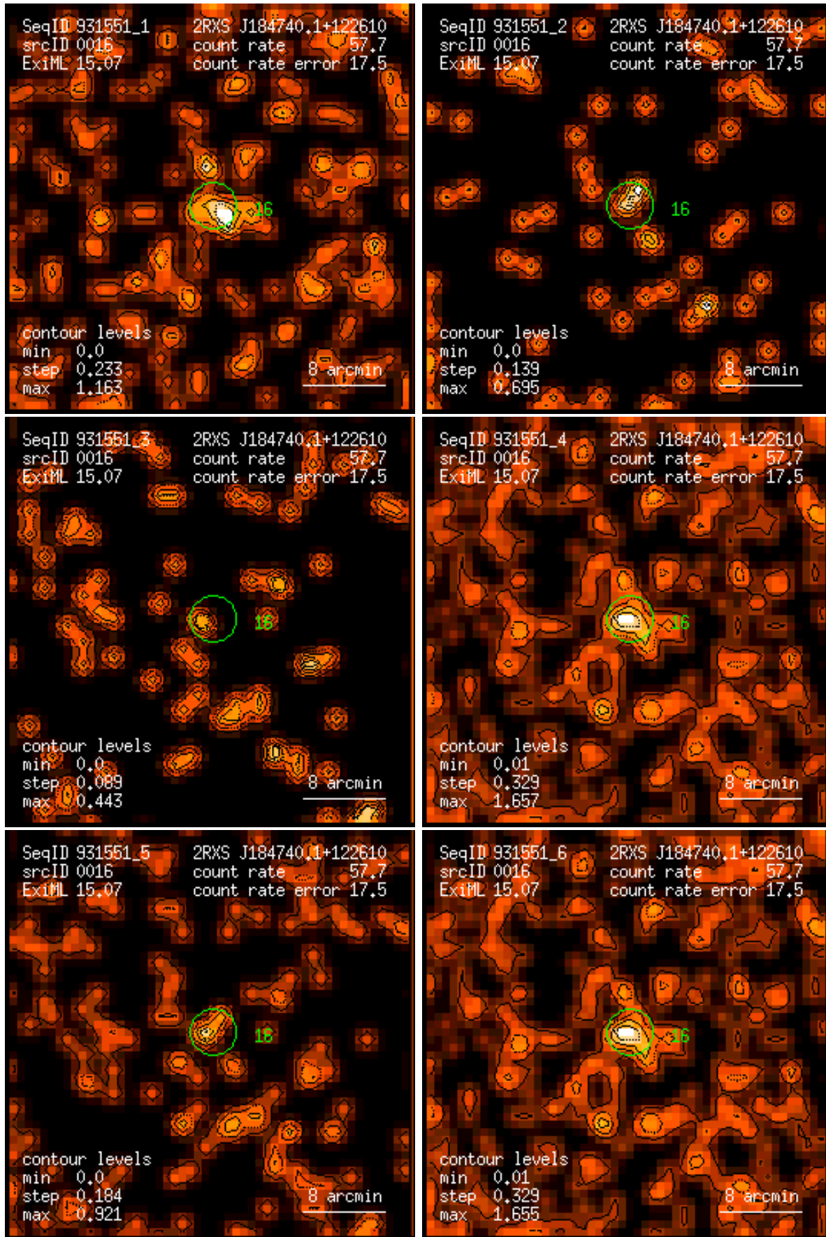
Figure 16: RASS 931551: detection 0016: band rate images, Gaussian filter: (1) PSPC channels 11 – 41, (2) 52 – 90, (3) 91 – 201, (4) 11 – 235, (5) 52 – 201, (6) 11 – 201. Broad band rates in counts/ks. Band rate contour levels in counts/ks/arcmin 2 .
