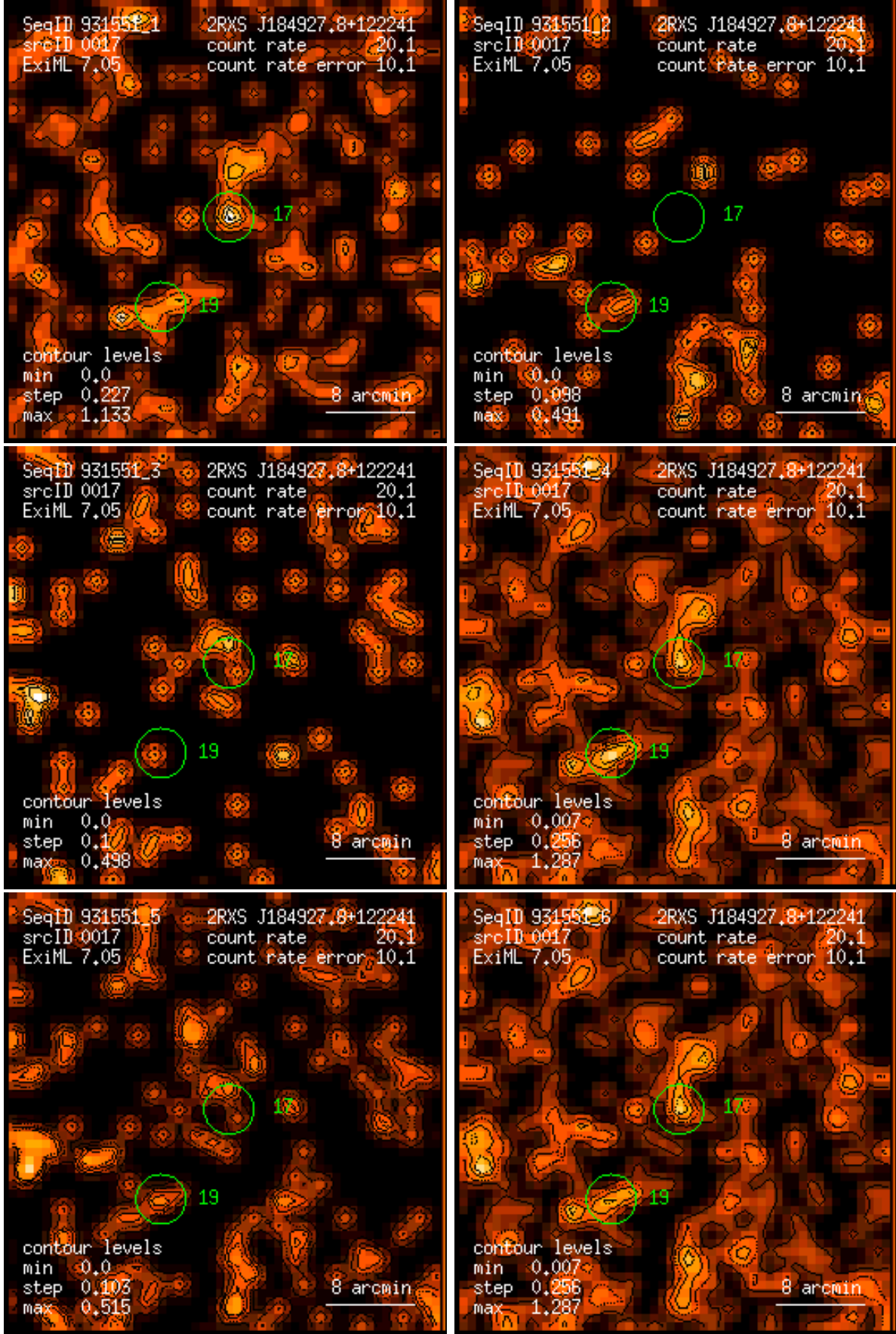
Figure 17: RASS 931551: detection 0017: band rate images, Gaussian filter: (1) PSPC channels 11 – 41, (2) 52 – 90, (3) 91 – 201, (4) 11 – 235, (5) 52 – 201, (6) 11 – 201. Broad band rates in counts/ks. Band rate contour levels in counts/ks/arcmin 2 .
