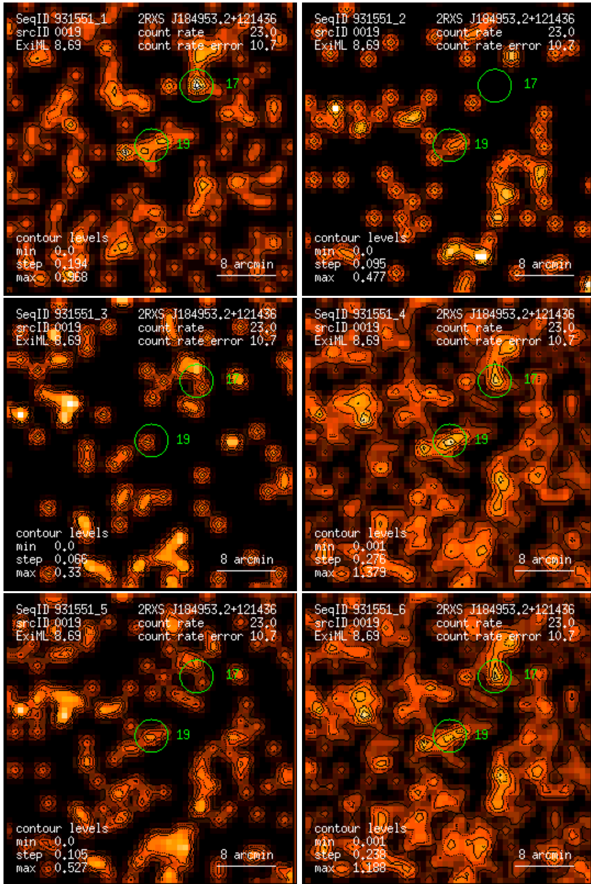
Figure 19: RASS 931551: detection 0019: band rate images, Gaussian filter: (1) PSPC channels 11 – 41, (2) 52 – 90, (3) 91 – 201, (4) 11 – 235, (5) 52 – 201, (6) 11 – 201. Broad band rates in counts/ks. Band rate contour levels in counts/ks/arcmin 2 .
