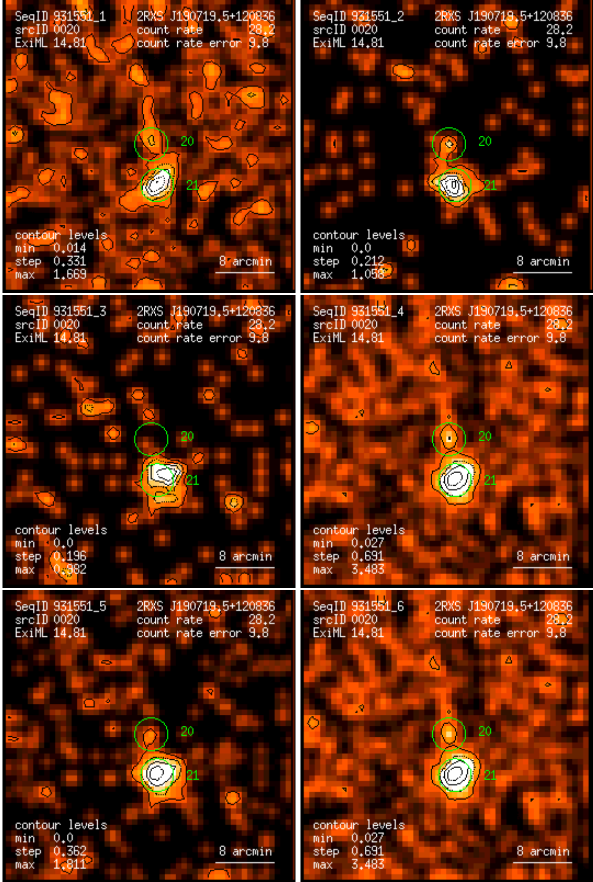
Figure 20: RASS 931551: detection 0020: band rate images, Gaussian filter: (1) PSPC channels 11 – 41, (2) 52 – 90, (3) 91 – 201, (4) 11 – 235, (5) 52 – 201, (6) 11 – 201. Broad band rates in counts/ks. Band rate contour levels in counts/ks/arcmin 2 .
