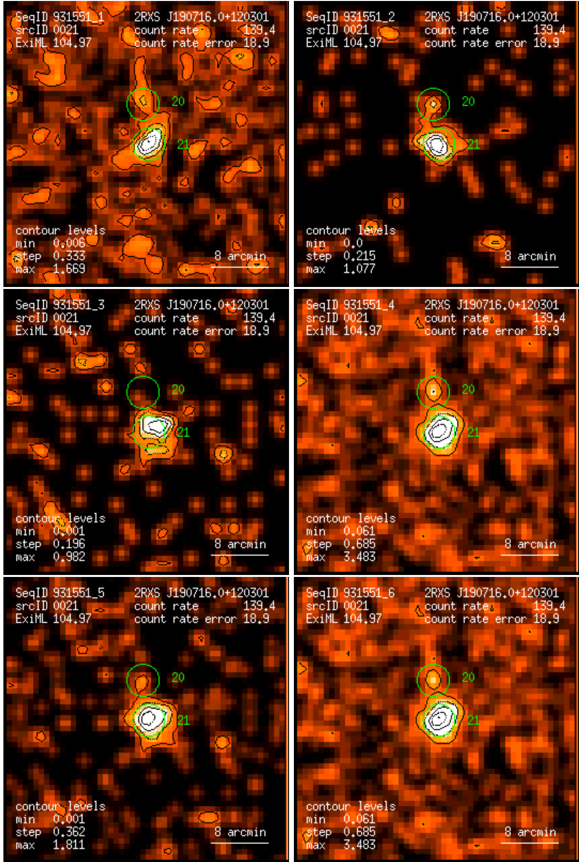
Figure 21: RASS 931551: detection 0021: band rate images, Gaussian filter: (1) PSPC channels 11 – 41, (2) 52 – 90, (3) 91 – 201, (4) 11 – 235, (5) 52 – 201, (6) 11 – 201. Broad band rates in counts/ks. Band rate contour levels in counts/ks/arcmin 2 .
