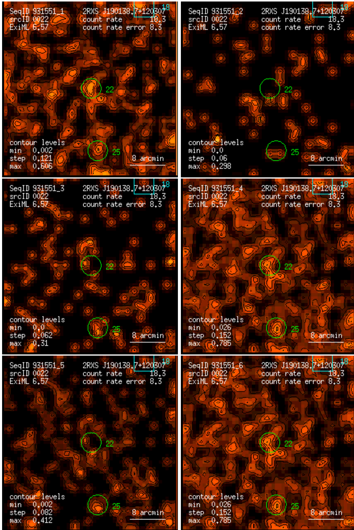
Figure 22: RASS 931551: detection 0022: band rate images, Gaussian filter: (1) PSPC channels 11 – 41, (2) 52 – 90, (3) 91 – 201, (4) 11 – 235, (5) 52 – 201, (6) 11 – 201. Broad band rates in counts/ks. Band rate contour levels in counts/ks/arcmin 2 .
