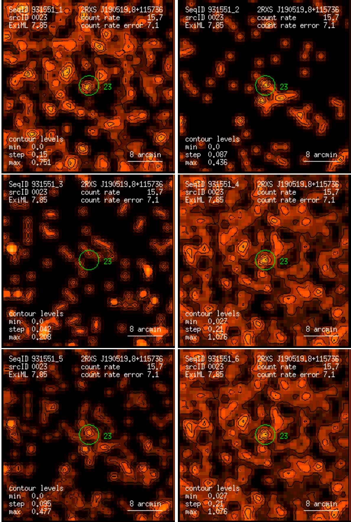
Figure 23: RASS 931551: detection 0023: band rate images, Gaussian filter: (1) PSPC channels 11 – 41, (2) 52 – 90, (3) 91 – 201, (4) 11 – 235, (5) 52 – 201, (6) 11 – 201. Broad band rates in counts/ks. Band rate contour levels in counts/ks/arcmin 2 .
