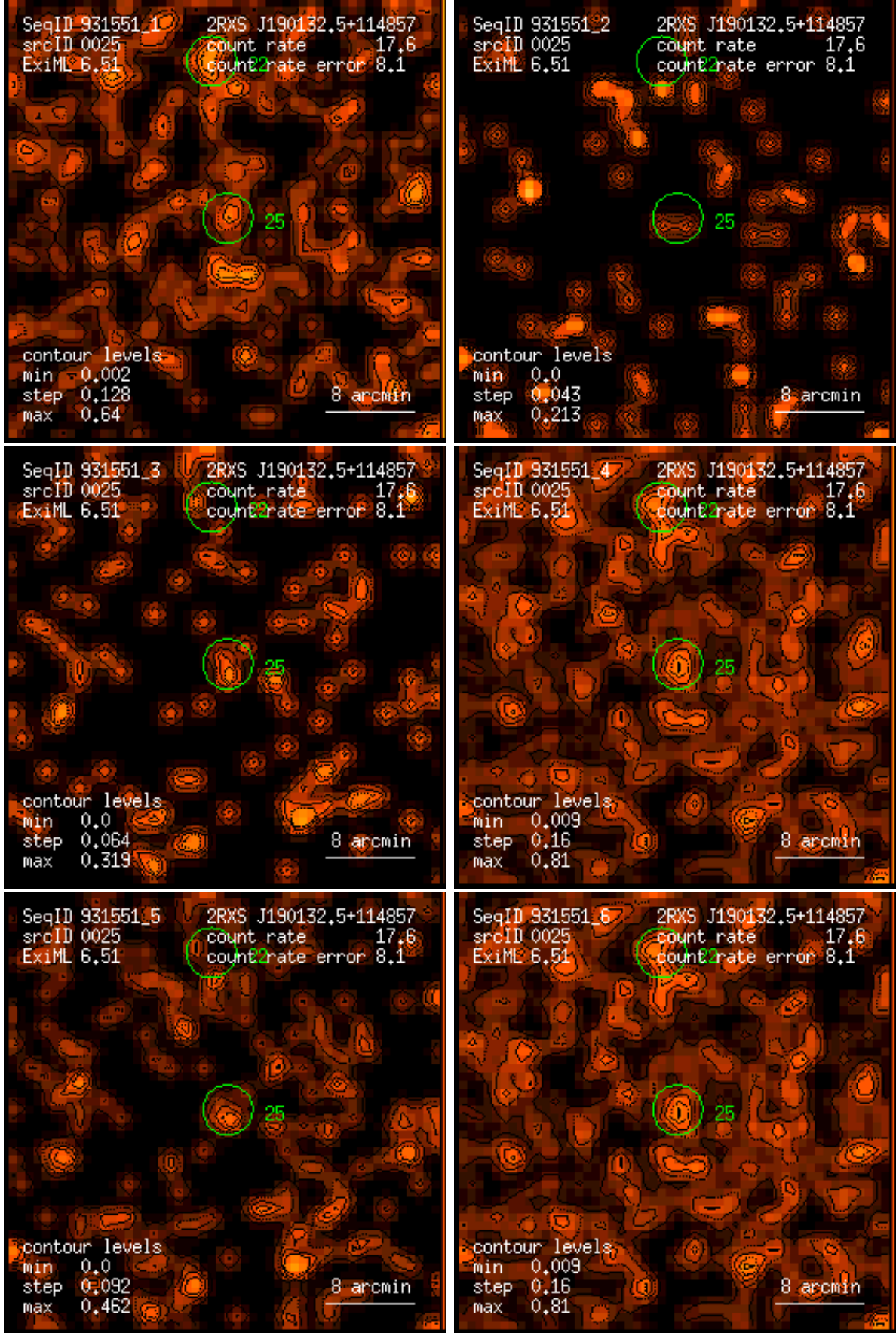
Figure 25: RASS 931551: detection 0025: band rate images, Gaussian filter: (1) PSPC channels 11 – 41, (2) 52 – 90, (3) 91 – 201, (4) 11 – 235, (5) 52 – 201, (6) 11 – 201. Broad band rates in counts/ks. Band rate contour levels in counts/ks/arcmin 2 .
