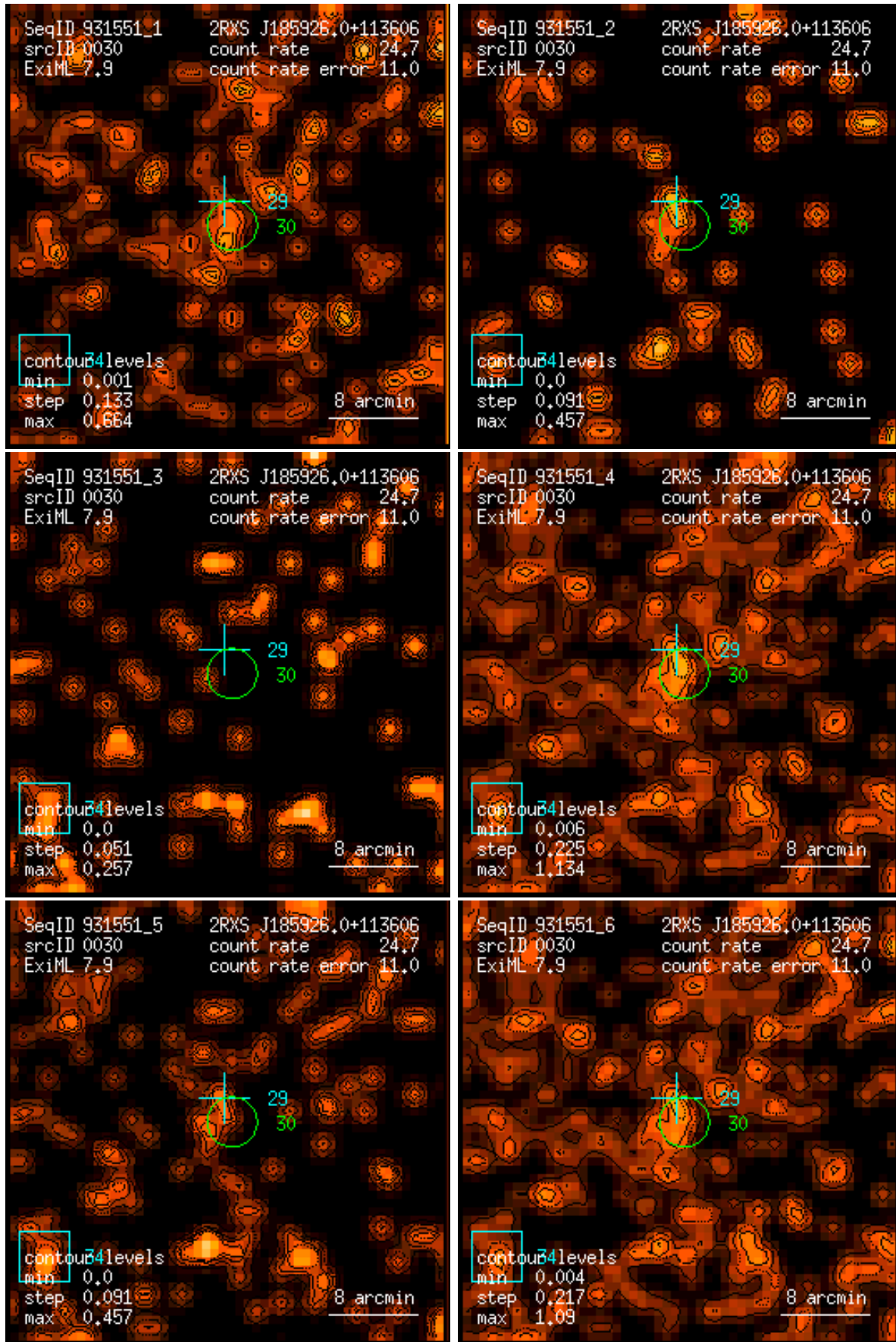
Figure 30: RASS 931551: detection 0030: band rate images, Gaussian filter: (1) PSPC channels 11 – 41, (2) 52 – 90, (3) 91 – 201, (4) 11 – 235, (5) 52 – 201, (6) 11 – 201. Broad band rates in counts/ks. Band rate contour levels in counts/ks/arcmin 2 .
