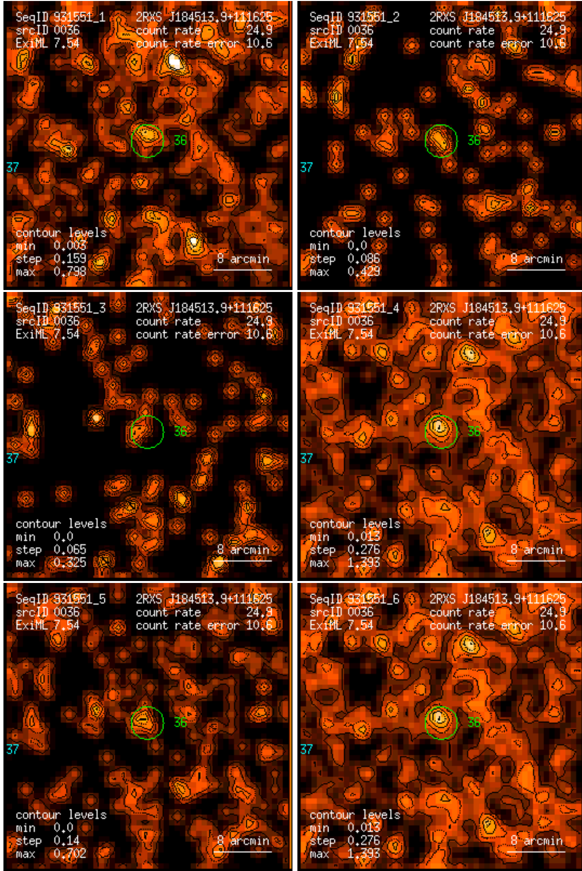
Figure 36: RASS 931551: detection 0036: band rate images, Gaussian filter: (1) PSPC channels 11 – 41, (2) 52 – 90, (3) 91 – 201, (4) 11 – 235, (5) 52 – 201, (6) 11 – 201. Broad band rates in counts/ks. Band rate contour levels in counts/ks/arcmin 2 .
