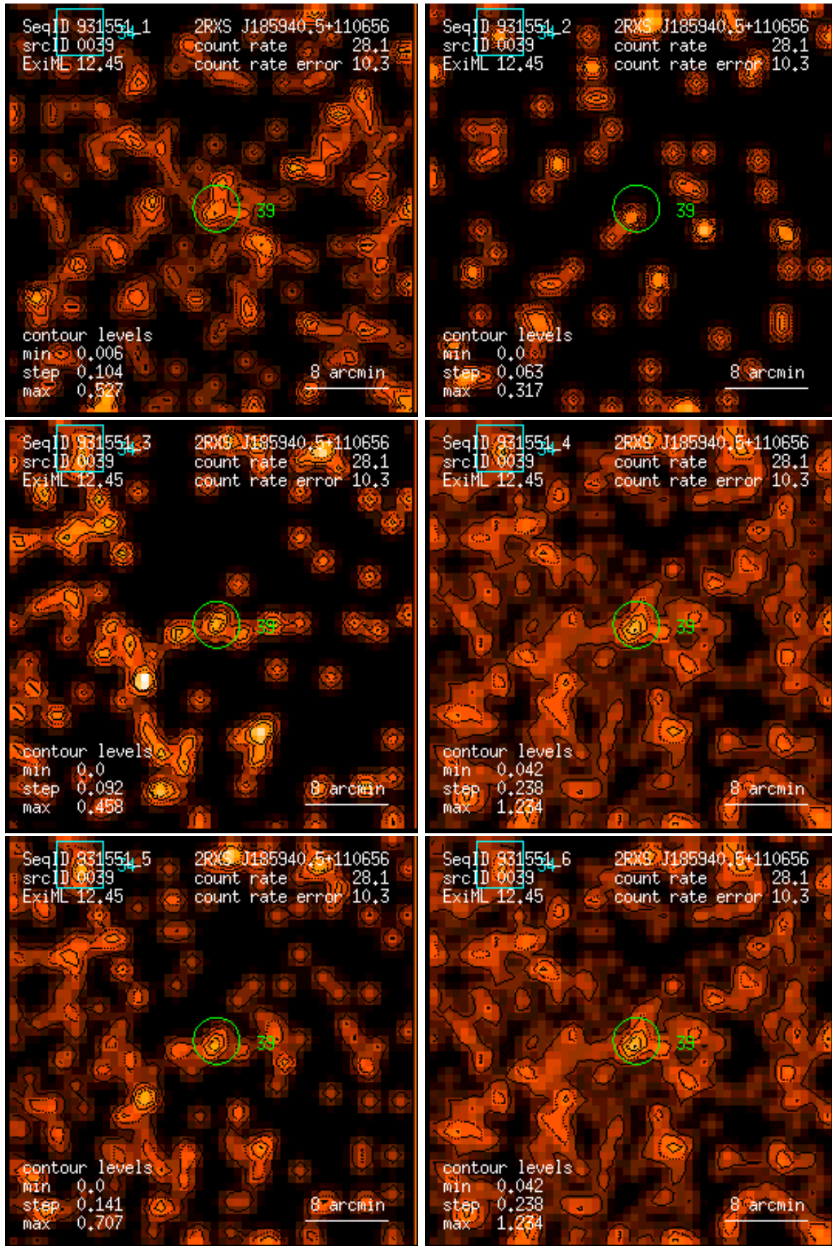
Figure 39: RASS 931551: detection 0039: band rate images, Gaussian filter: (1) PSPC channels 11 – 41, (2) 52 – 90, (3) 91 – 201, (4) 11 – 235, (5) 52 – 201, (6) 11 – 201. Broad band rates in counts/ks. Band rate contour levels in counts/ks/arcmin 2 .
