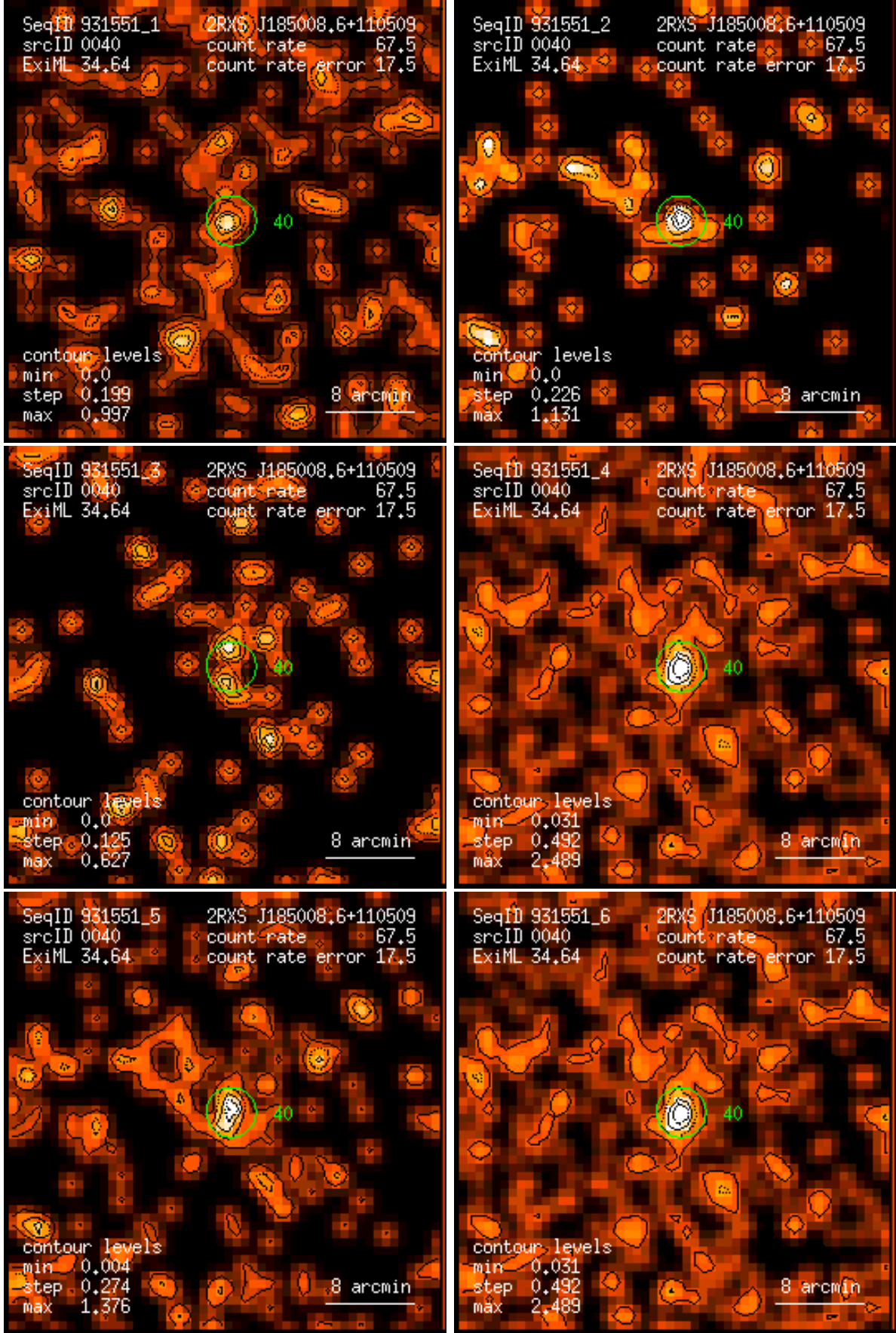
Figure 40: RASS 931551: detection 0040: band rate images, Gaussian filter: (1) PSPC channels 11 – 41, (2) 52 – 90, (3) 91 – 201, (4) 11 – 235, (5) 52 – 201, (6) 11 – 201. Broad band rates in counts/ks. Band rate contour levels in counts/ks/arcmin 2 .
