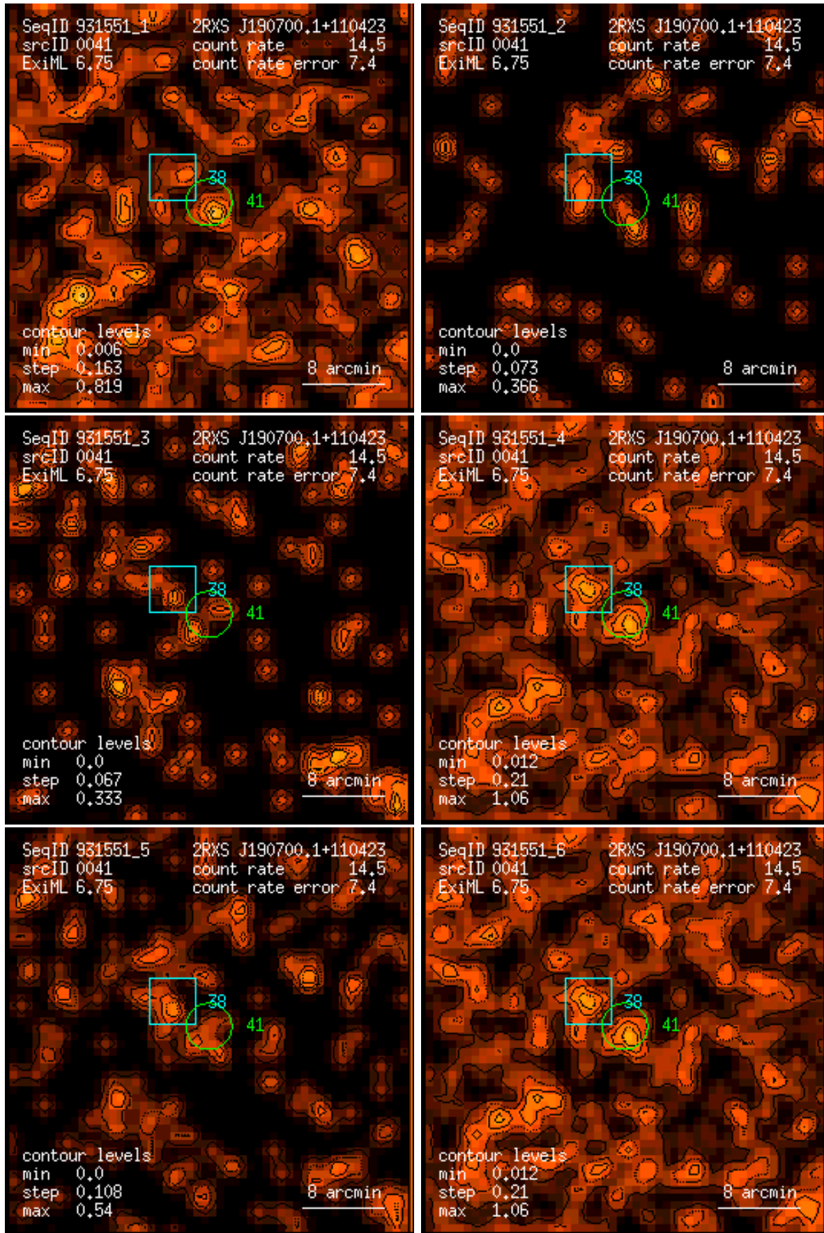
Figure 41: RASS 931551: detection 0041: band rate images, Gaussian filter: (1) PSPC channels 11 – 41, (2) 52 – 90, (3) 91 – 201, (4) 11 – 235, (5) 52 – 201, (6) 11 – 201. Broad band rates in counts/ks. Band rate contour levels in counts/ks/arcmin 2 .
