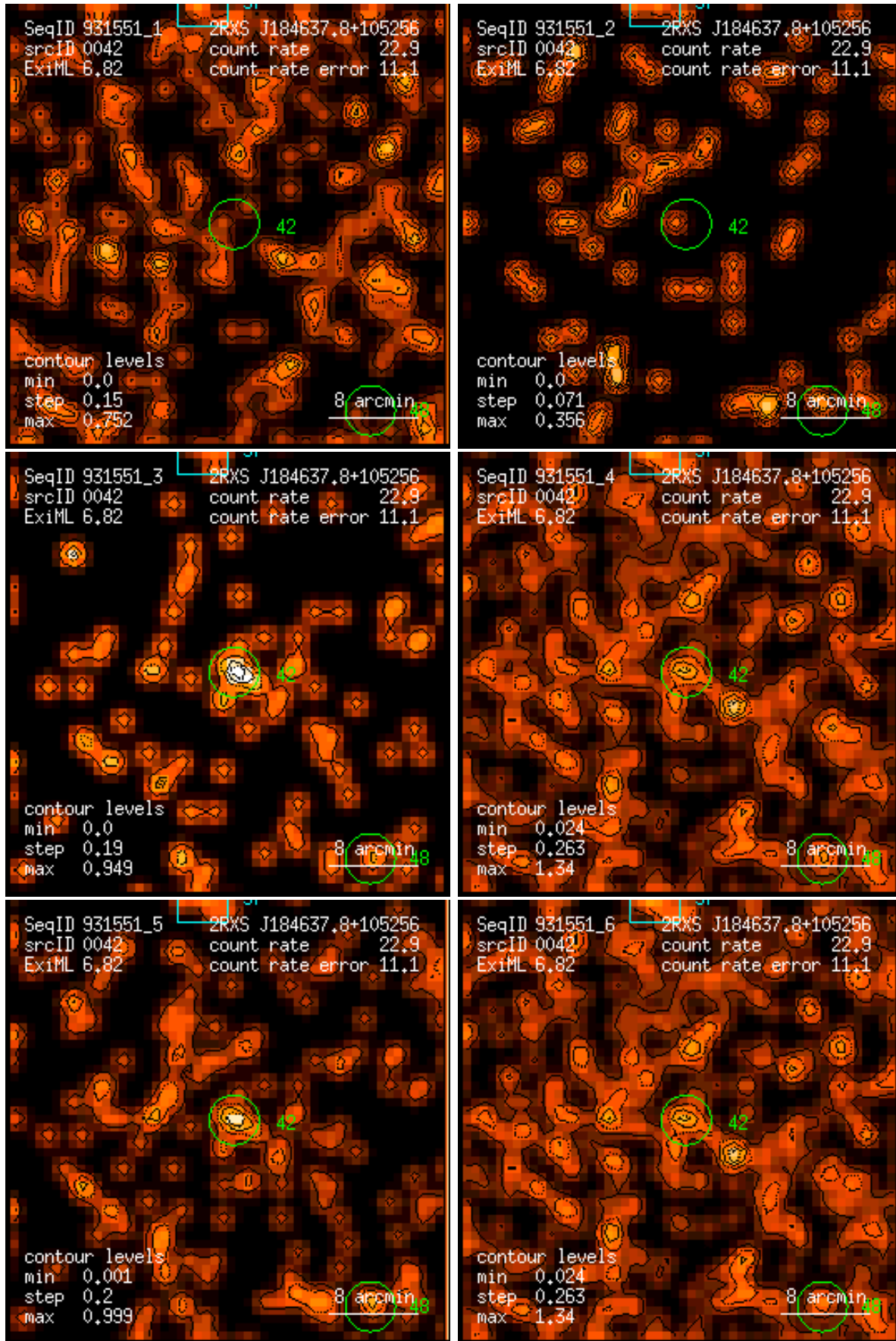
Figure 42: RASS 931551: detection 0042: band rate images, Gaussian filter: (1) PSPC channels 11 – 41, (2) 52 – 90, (3) 91 – 201, (4) 11 – 235, (5) 52 – 201, (6) 11 – 201. Broad band rates in counts/ks. Band rate contour levels in counts/ks/arcmin 2 .
