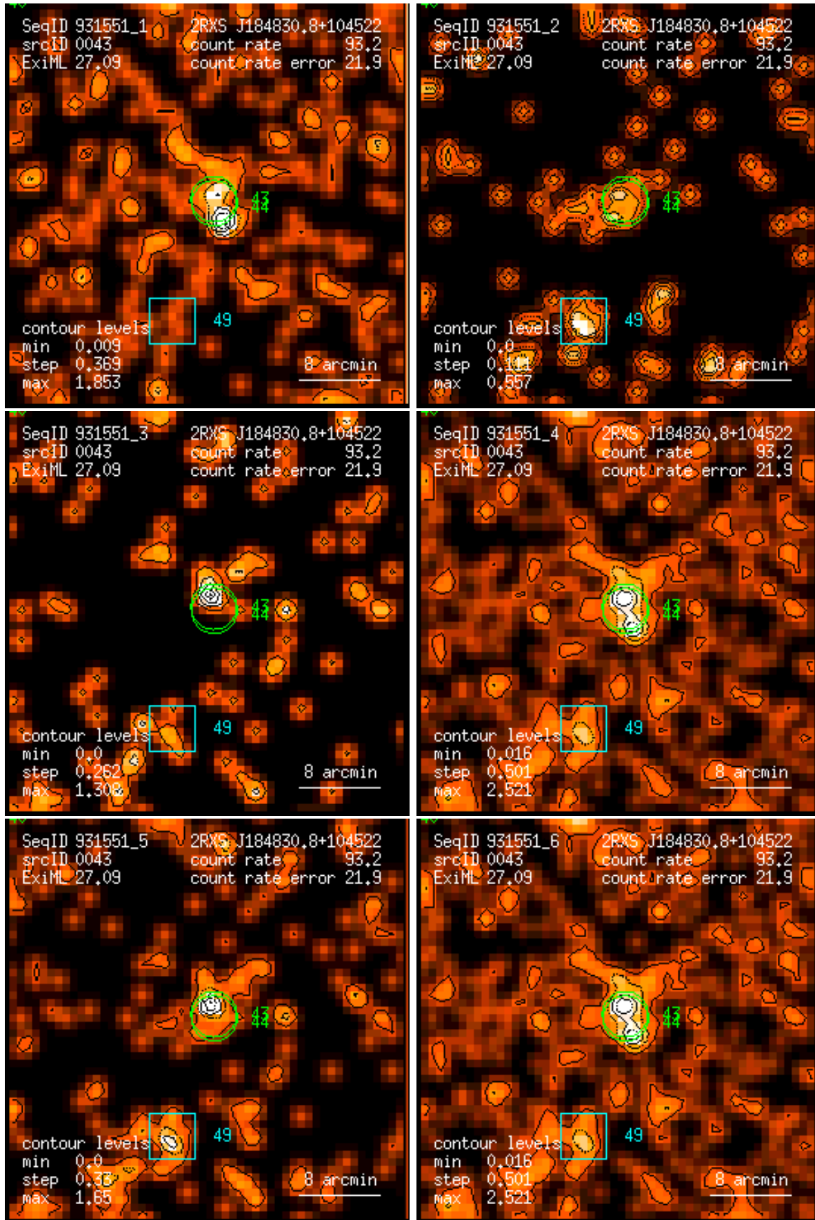
Figure 43: RASS 931551: detection 0043: band rate images, Gaussian filter: (1) PSPC channels 11 – 41, (2) 52 – 90, (3) 91 – 201, (4) 11 – 235, (5) 52 – 201, (6) 11 – 201. Broad band rates in counts/ks. Band rate contour levels in counts/ks/arcmin 2 .
