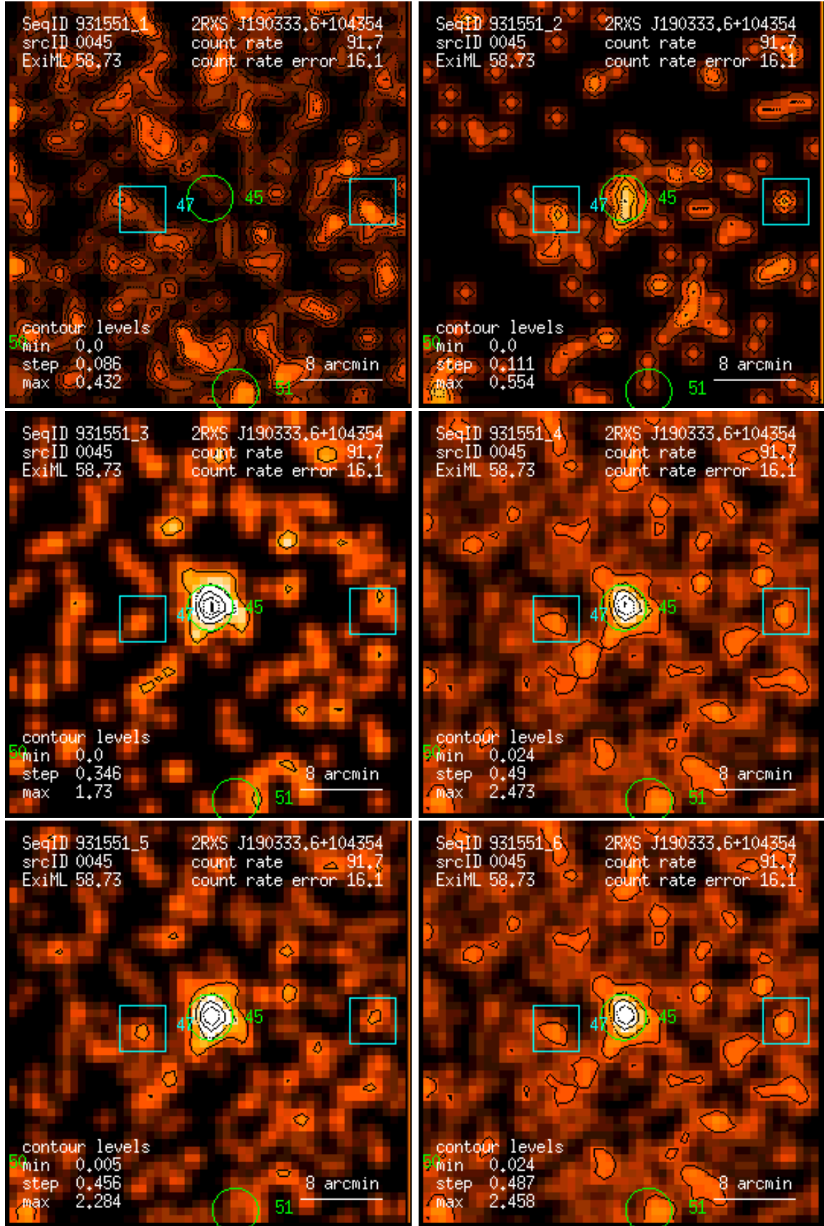
Figure 45: RASS 931551: detection 0045: band rate images, Gaussian filter: (1) PSPC channels 11 – 41, (2) 52 – 90, (3) 91 – 201, (4) 11 – 235, (5) 52 – 201, (6) 11 – 201. Broad band rates in counts/ks. Band rate contour levels in counts/ks/arcmin 2 .
