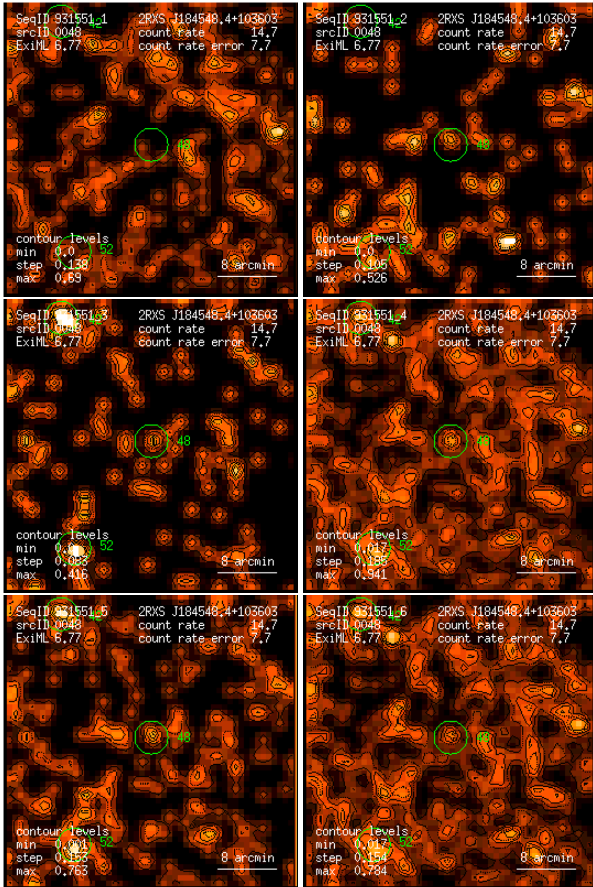
Figure 48: RASS 931551: detection 0048: band rate images, Gaussian filter: (1) PSPC channels 11 – 41, (2) 52 – 90, (3) 91 – 201, (4) 11 – 235, (5) 52 – 201, (6) 11 – 201. Broad band rates in counts/ks. Band rate contour levels in counts/ks/arcmin 2 .
