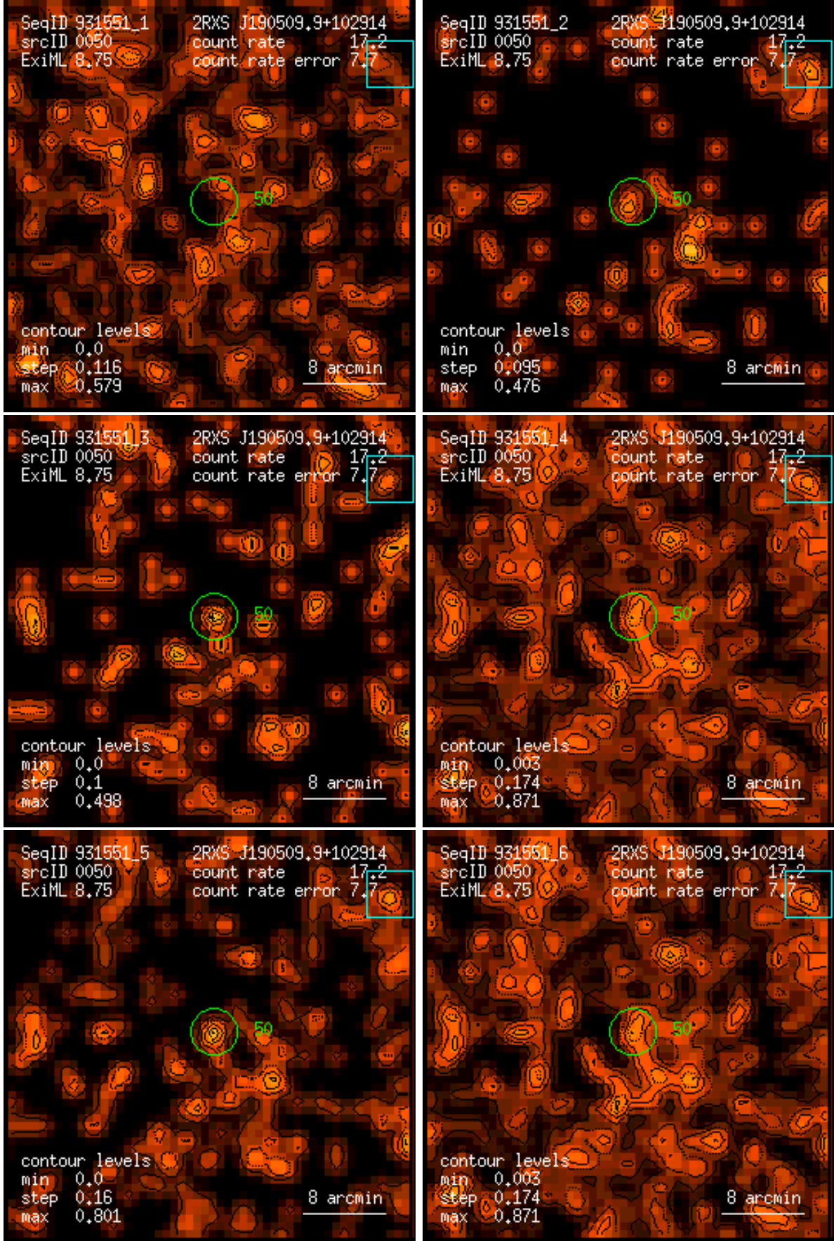
Figure 50: RASS 931551: detection 0050: band rate images, Gaussian filter: (1) PSPC channels 11 – 41, (2) 52 – 90, (3) 91 – 201, (4) 11 – 235, (5) 52 – 201, (6) 11 – 201. Broad band rates in counts/ks. Band rate contour levels in counts/ks/arcmin 2 .
