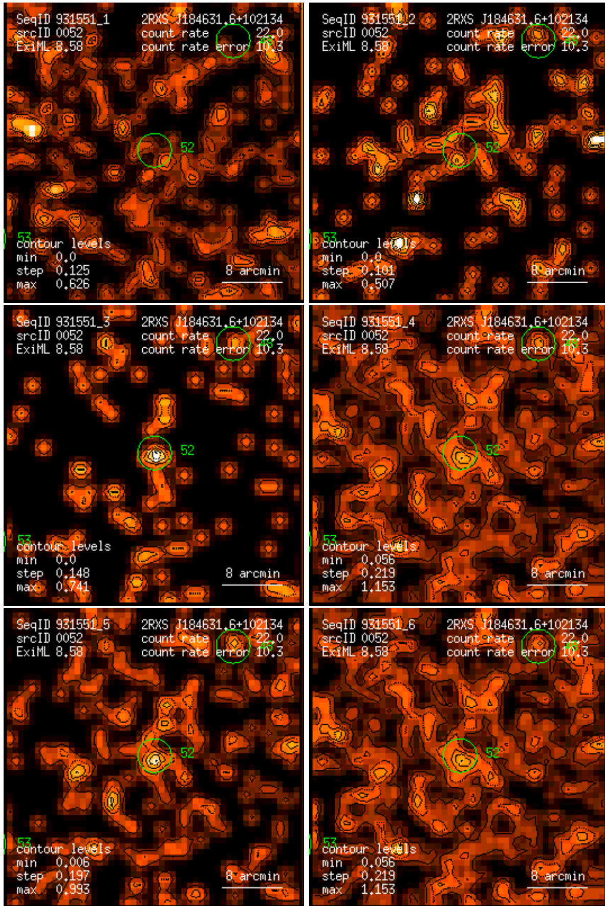
Figure 52: RASS 931551: detection 0052: band rate images, Gaussian filter: (1) PSPC channels 11 – 41, (2) 52 – 90, (3) 91 – 201, (4) 11 – 235, (5) 52 – 201, (6) 11 – 201. Broad band rates in counts/ks. Band rate contour levels in counts/ks/arcmin 2 .
