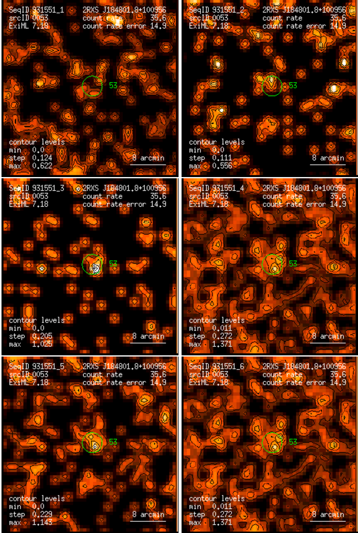
Figure 53: RASS 931551: detection 0053: band rate images, Gaussian filter: (1) PSPC channels 11 – 41, (2) 52 – 90, (3) 91 – 201, (4) 11 – 235, (5) 52 – 201, (6) 11 – 201. Broad band rates in counts/ks. Band rate contour levels in counts/ks/arcmin 2 .
