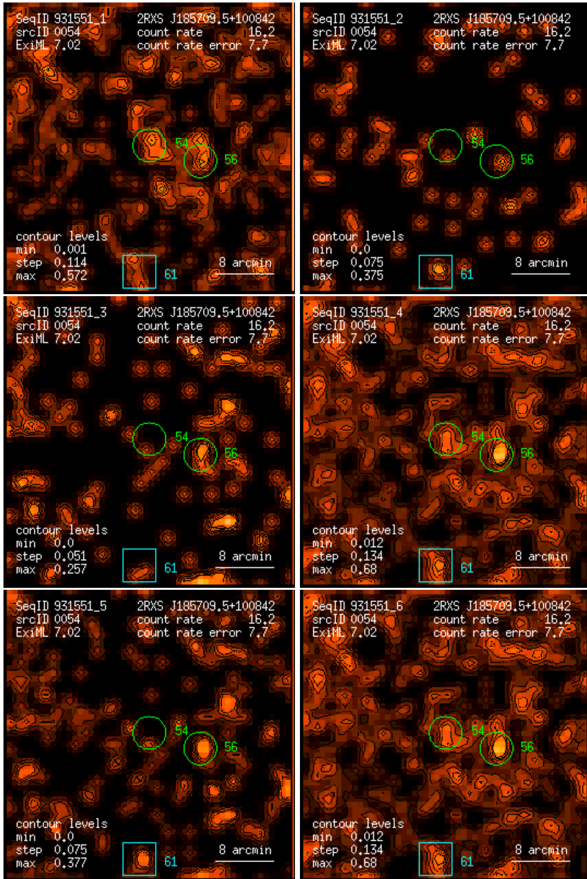
Figure 54: RASS 931551: detection 0054: band rate images, Gaussian filter: (1) PSPC channels 11 – 41, (2) 52 – 90, (3) 91 – 201, (4) 11 – 235, (5) 52 – 201, (6) 11 – 201. Broad band rates in counts/ks. Band rate contour levels in counts/ks/arcmin 2 .
