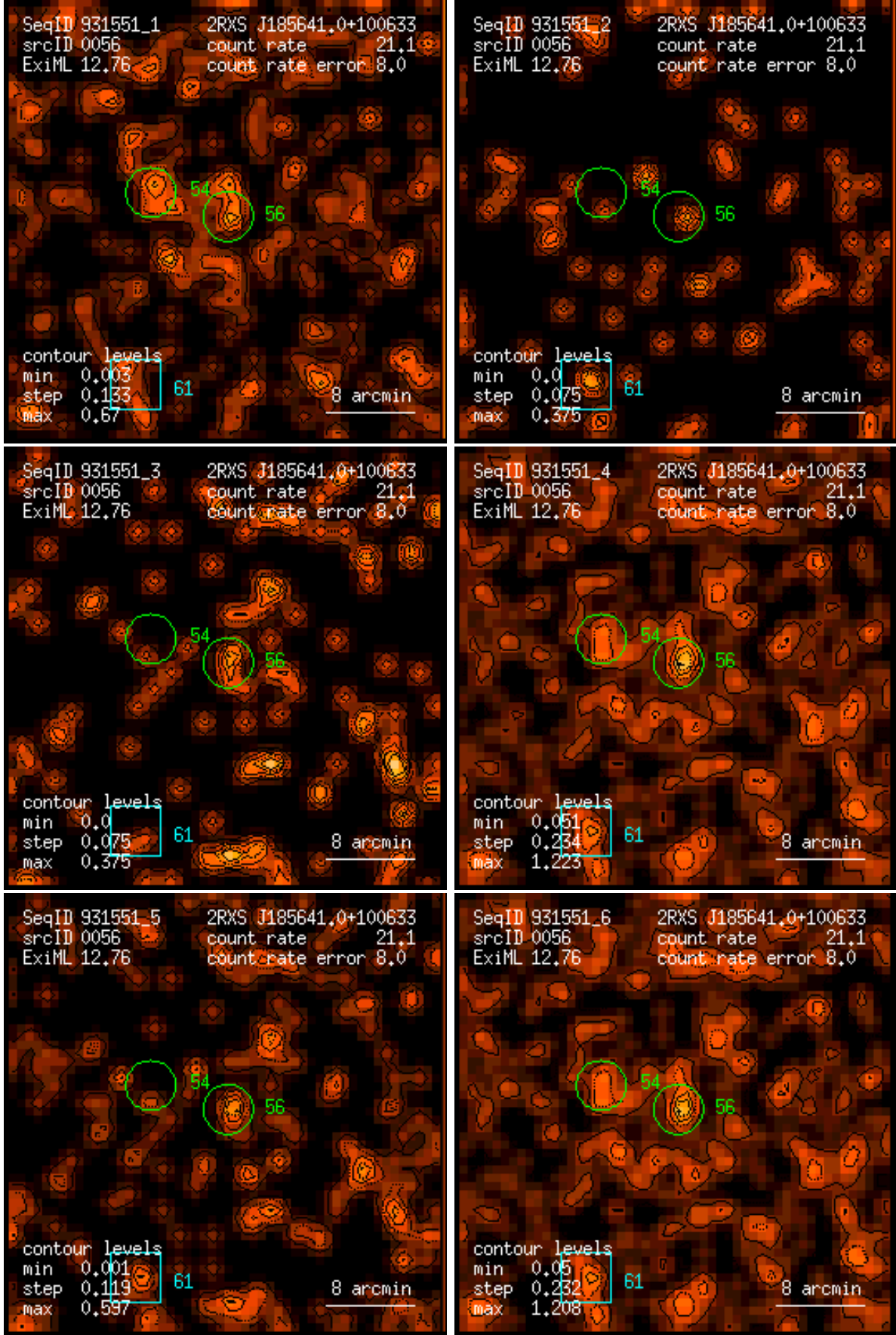
Figure 56: RASS 931551: detection 0056: band rate images, Gaussian filter: (1) PSPC channels 11 – 41, (2) 52 – 90, (3) 91 – 201, (4) 11 – 235, (5) 52 – 201, (6) 11 – 201. Broad band rates in counts/ks. Band rate contour levels in counts/ks/arcmin 2 .
