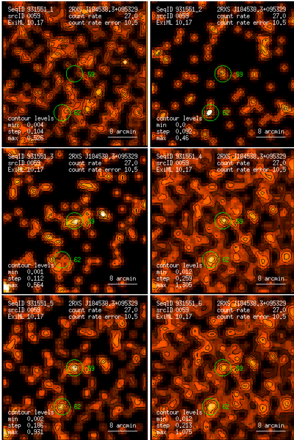
Figure 59: RASS 931551: detection 0059: band rate images, Gaussian filter: (1) PSPC channels 11 – 41, (2) 52 – 90, (3) 91 – 201, (4) 11 – 235, (5) 52 – 201, (6) 11 – 201. Broad band rates in counts/ks. Band rate contour levels in counts/ks/arcmin 2 .
