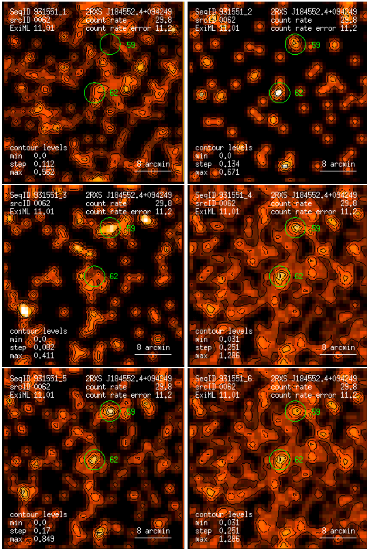
Figure 62: RASS 931551: detection 0062: band rate images, Gaussian filter: (1) PSPC channels 11 – 41, (2) 52 – 90, (3) 91 – 201, (4) 11 – 235, (5) 52 – 201, (6) 11 – 201. Broad band rates in counts/ks. Band rate contour levels in counts/ks/arcmin 2 .
