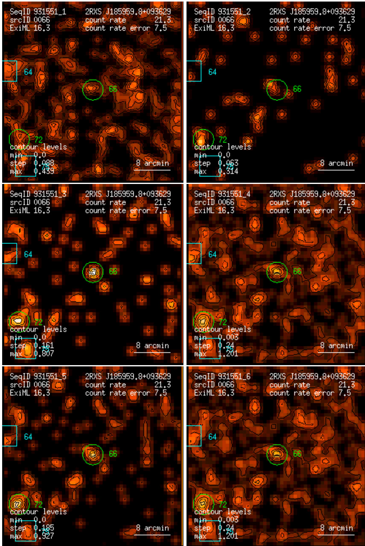
Figure 66: RASS 931551: detection 0066: band rate images, Gaussian filter: (1) PSPC channels 11 – 41, (2) 52 – 90, (3) 91 – 201, (4) 11 – 235, (5) 52 – 201, (6) 11 – 201. Broad band rates in counts/ks. Band rate contour levels in counts/ks/arcmin 2 .
