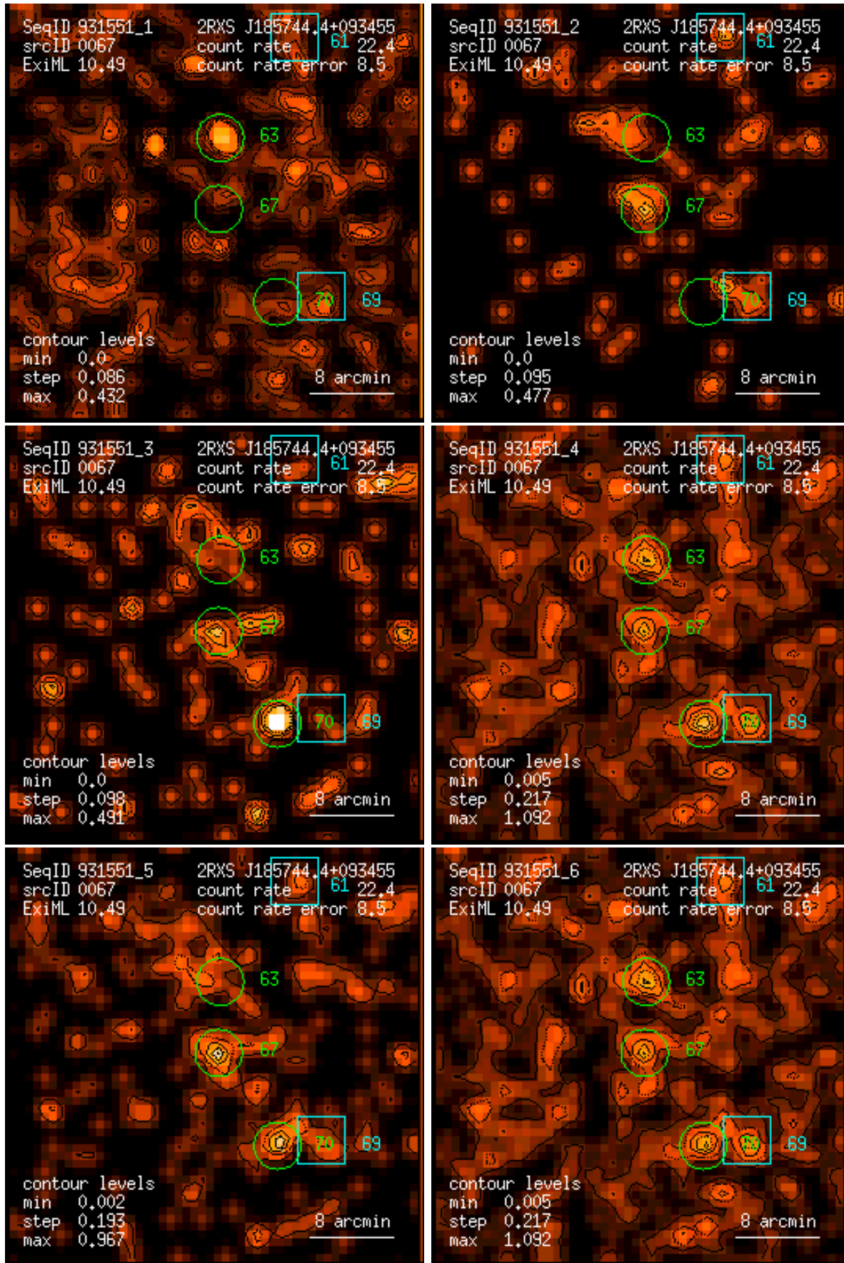
Figure 67: RASS 931551: detection 0067: band rate images, Gaussian filter: (1) PSPC channels 11 – 41, (2) 52 – 90, (3) 91 – 201, (4) 11 – 235, (5) 52 – 201, (6) 11 – 201. Broad band rates in counts/ks. Band rate contour levels in counts/ks/arcmin 2 .
