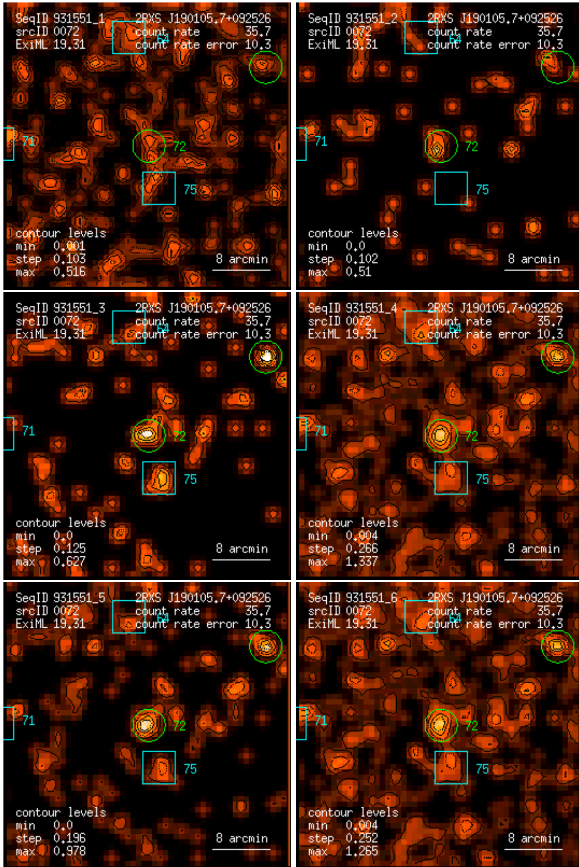
Figure 72: RASS 931551: detection 0072: band rate images, Gaussian filter: (1) PSPC channels 11 – 41, (2) 52 – 90, (3) 91 – 201, (4) 11 – 235, (5) 52 – 201, (6) 11 – 201. Broad band rates in counts/ks. Band rate contour levels in counts/ks/arcmin 2 .
