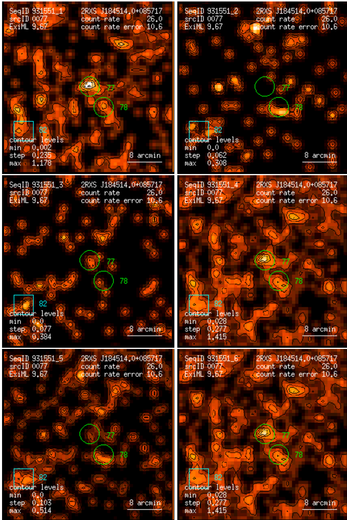
Figure 77: RASS 931551: detection 0077: band rate images, Gaussian filter: (1) PSPC channels 11 – 41, (2) 52 – 90, (3) 91 – 201, (4) 11 – 235, (5) 52 – 201, (6) 11 – 201. Broad band rates in counts/ks. Band rate contour levels in counts/ks/arcmin 2 .
