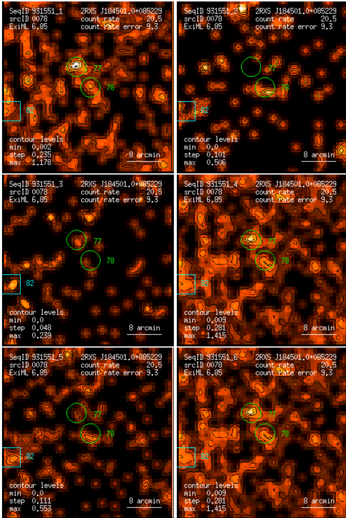
Figure 78: RASS 931551: detection 0078: band rate images, Gaussian filter: (1) PSPC channels 11 – 41, (2) 52 – 90, (3) 91 – 201, (4) 11 – 235, (5) 52 – 201, (6) 11 – 201. Broad band rates in counts/ks. Band rate contour levels in counts/ks/arcmin 2 .
