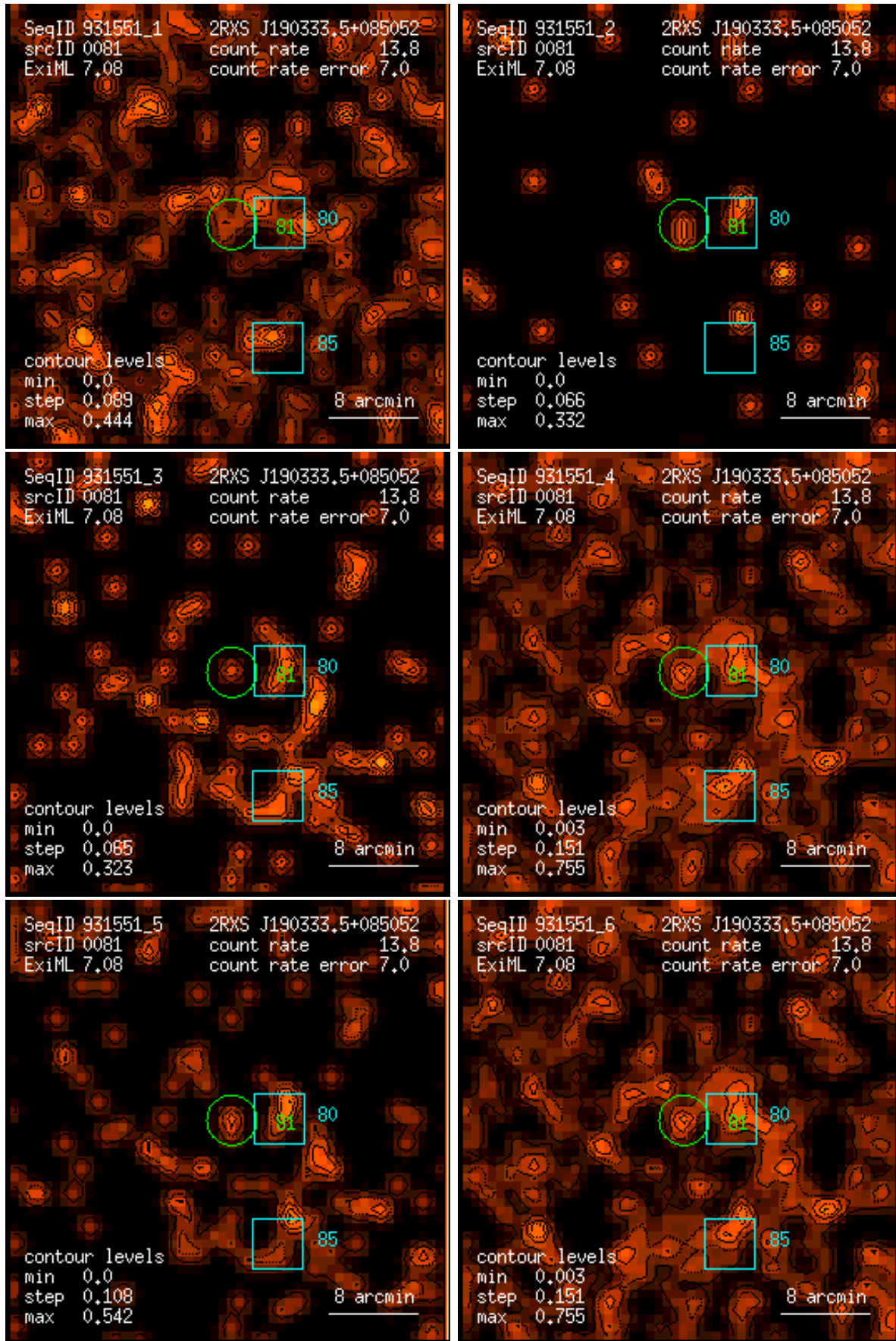
Figure 81: RASS 931551: detection 0081: band rate images, Gaussian filter: (1) PSPC channels 11 – 41, (2) 52 – 90, (3) 91 – 201, (4) 11 – 235, (5) 52 – 201, (6) 11 – 201. Broad band rates in counts/ks. Band rate contour levels in counts/ks/arcmin 2 .
