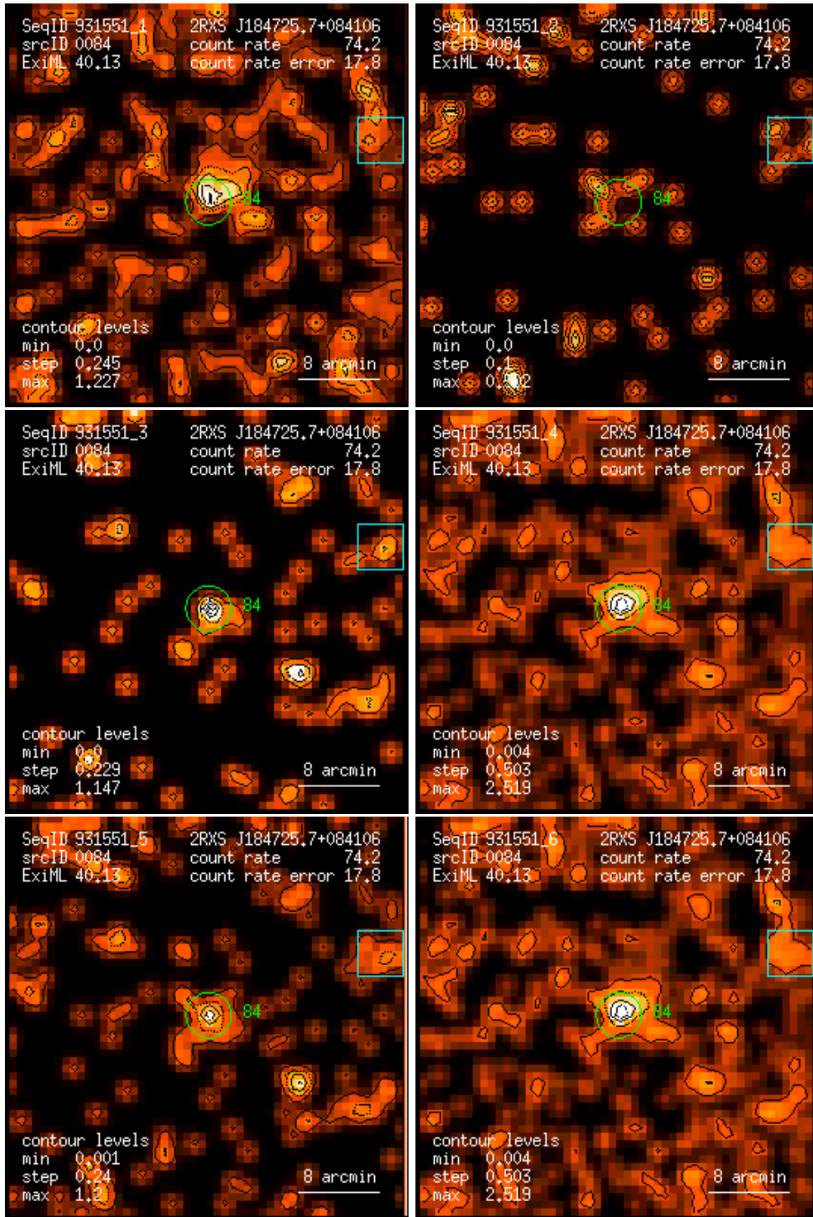
Figure 84: RASS 931551: detection 0084: band rate images, Gaussian filter: (1) PSPC channels 11 – 41, (2) 52 – 90, (3) 91 – 201, (4) 11 – 235, (5) 52 – 201, (6) 11 – 201. Broad band rates in counts/ks. Band rate contour levels in counts/ks/arcmin 2 .
