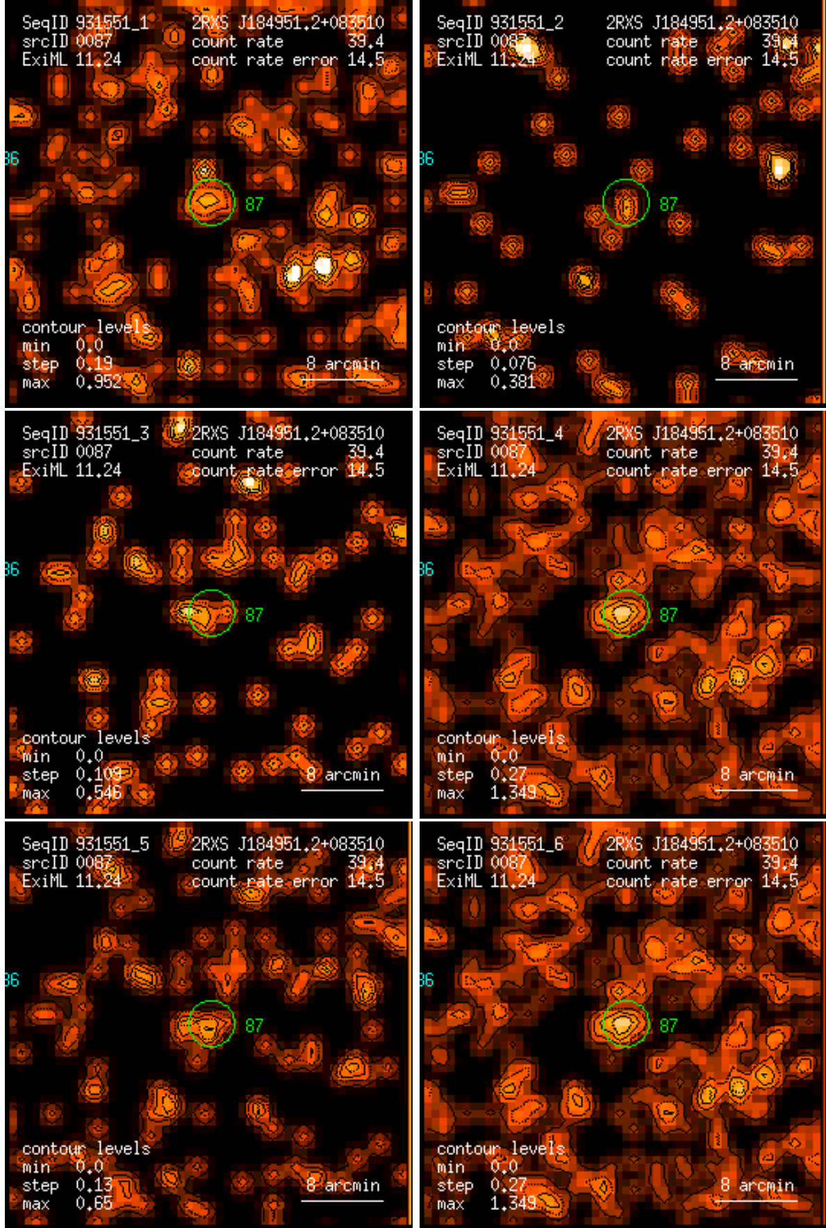
Figure 87: RASS 931551: detection 0087: band rate images, Gaussian filter: (1) PSPC channels 11 – 41, (2) 52 – 90, (3) 91 – 201, (4) 11 – 235, (5) 52 – 201, (6) 11 – 201. Broad band rates in counts/ks. Band rate contour levels in counts/ks/arcmin 2 .
