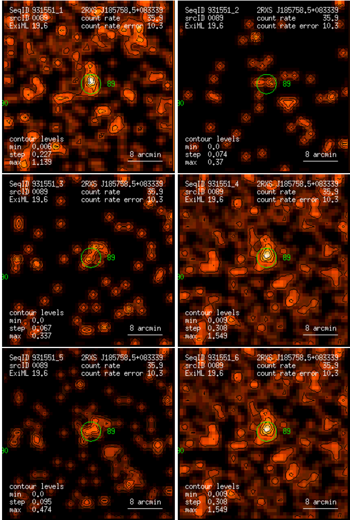
Figure 89: RASS 931551: detection 0089: band rate images, Gaussian filter: (1) PSPC channels 11 – 41, (2) 52 – 90, (3) 91 – 201, (4) 11 – 235, (5) 52 – 201, (6) 11 – 201. Broad band rates in counts/ks. Band rate contour levels in counts/ks/arcmin 2 .
