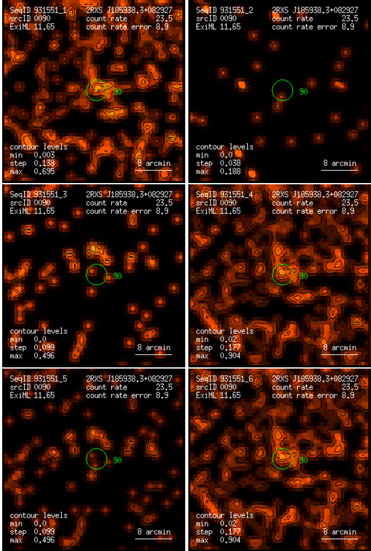
Figure 90: RASS 931551: detection 0090: band rate images, Gaussian filter: (1) PSPC channels 11 – 41, (2) 52 – 90, (3) 91 – 201, (4) 11 – 235, (5) 52 – 201, (6) 11 – 201. Broad band rates in counts/ks. Band rate contour levels in counts/ks/arcmin 2 .
