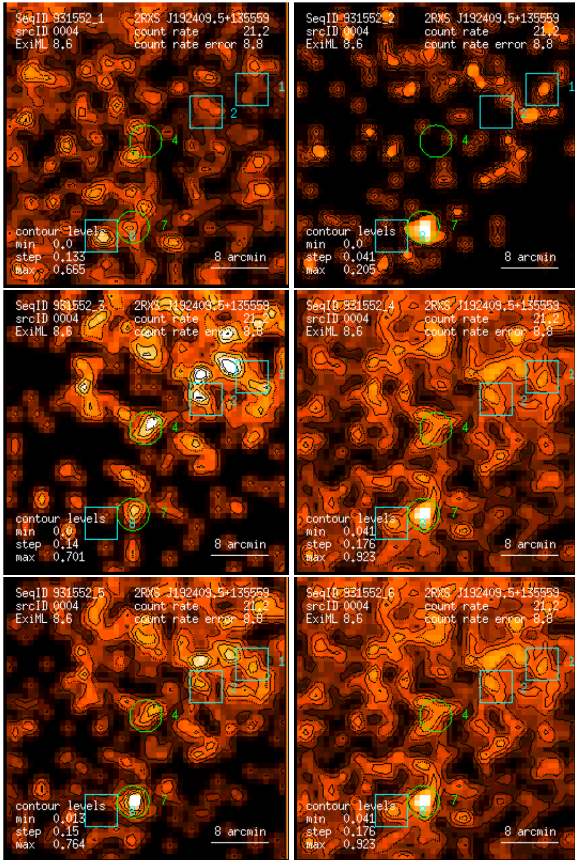
Figure 4: RASS 931552: detection 0004: band rate images, Gaussian filter: (1) PSPC channels 11 – 41, (2) 52 – 90, (3) 91 – 201, (4) 11 – 235, (5) 52 – 201, (6) 11 – 201. Broad band rates in counts/ks. Band rate contour levels in counts/ks/arcmin 2 .
