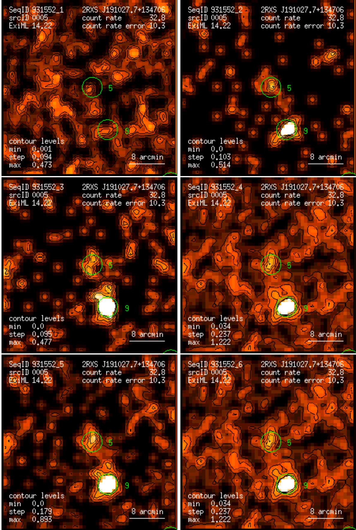
Figure 5: RASS 931552: detection 0005: band rate images, Gaussian filter: (1) PSPC channels 11 – 41, (2) 52 – 90, (3) 91 – 201, (4) 11 – 235, (5) 52 – 201, (6) 11 – 201. Broad band rates in counts/ks. Band rate contour levels in counts/ks/arcmin 2 .
