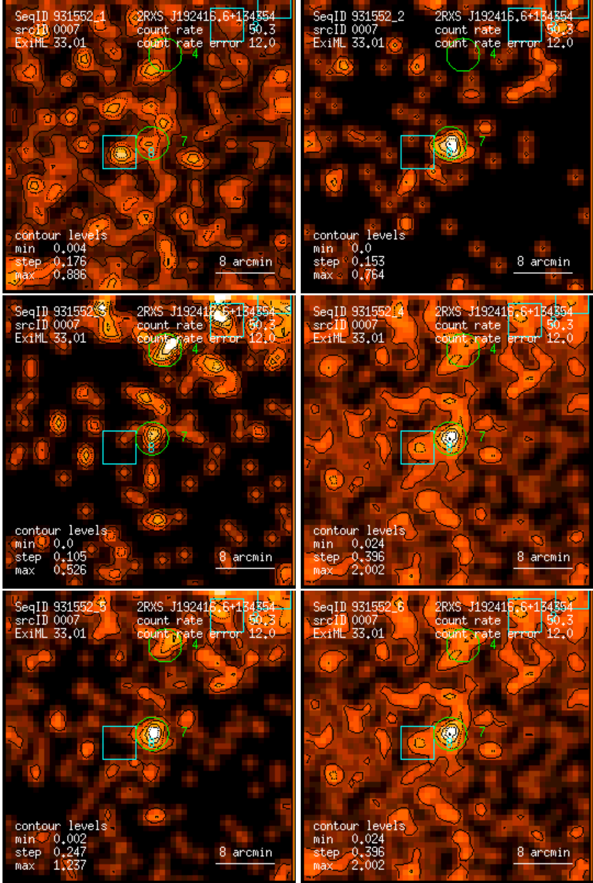
Figure 7: RASS 931552: detection 0007: band rate images, Gaussian filter: (1) PSPC channels 11 – 41, (2) 52 – 90, (3) 91 – 201, (4) 11 – 235, (5) 52 – 201, (6) 11 – 201. Broad band rates in counts/ks. Band rate contour levels in counts/ks/arcmin 2 .
