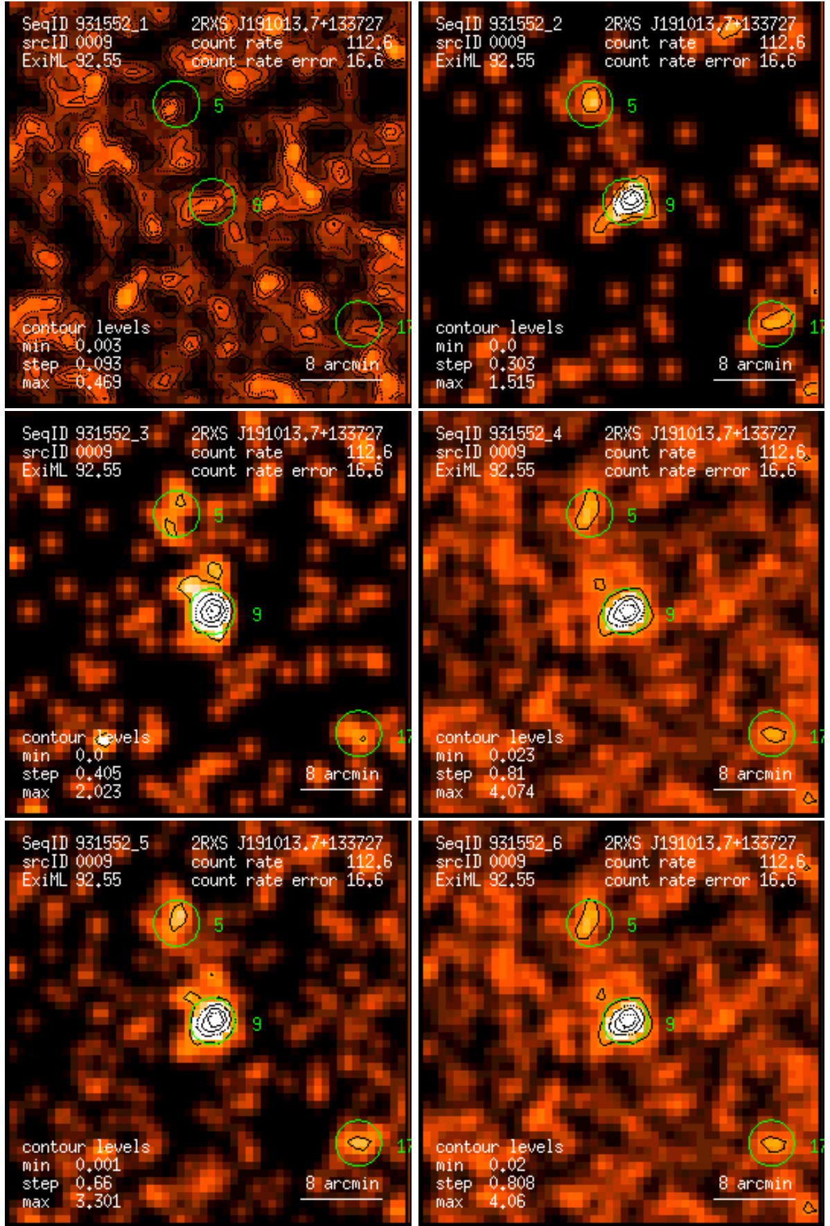
Figure 9: RASS 931552: detection 0009: band rate images, Gaussian filter: (1) PSPC channels 11 – 41, (2) 52 – 90, (3) 91 – 201, (4) 11 – 235, (5) 52 – 201, (6) 11 – 201. Broad band rates in counts/ks. Band rate contour levels in counts/ks/arcmin 2 .
