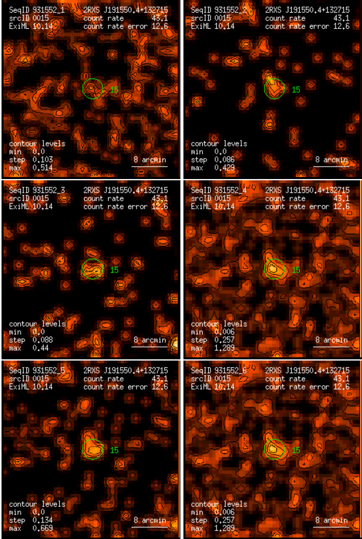
Figure 15: RASS 931552: detection 0015: band rate images, Gaussian filter: (1) PSPC channels 11 – 41, (2) 52 – 90, (3) 91 – 201, (4) 11 – 235, (5) 52 – 201, (6) 11 – 201. Broad band rates in counts/ks. Band rate contour levels in counts/ks/arcmin 2 .
